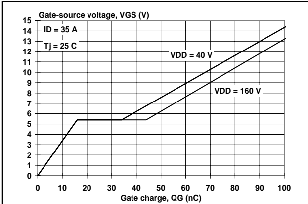
Fig.13. Typical turn-on gate-charge characteristics. V_{GS} = f(Q_G)
