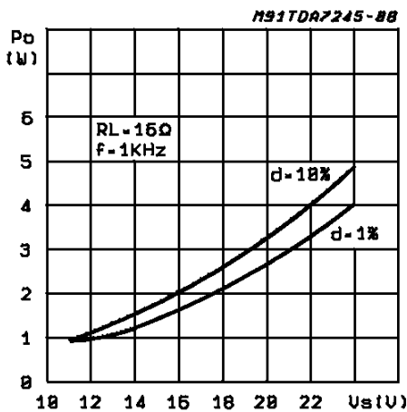
Figure 8: Output Power vs. Supply Voltage
