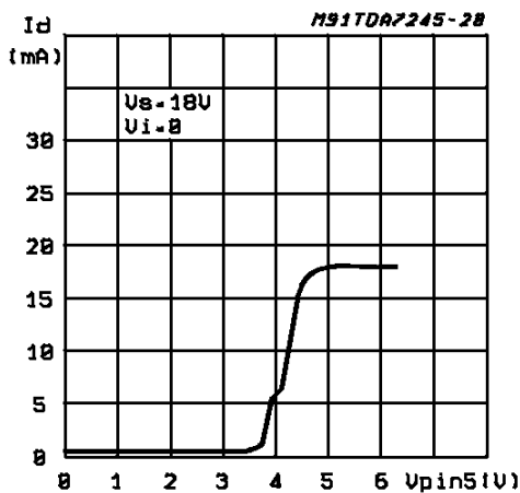
Figure 20: Quiescent Current vs. V_{pin5}
