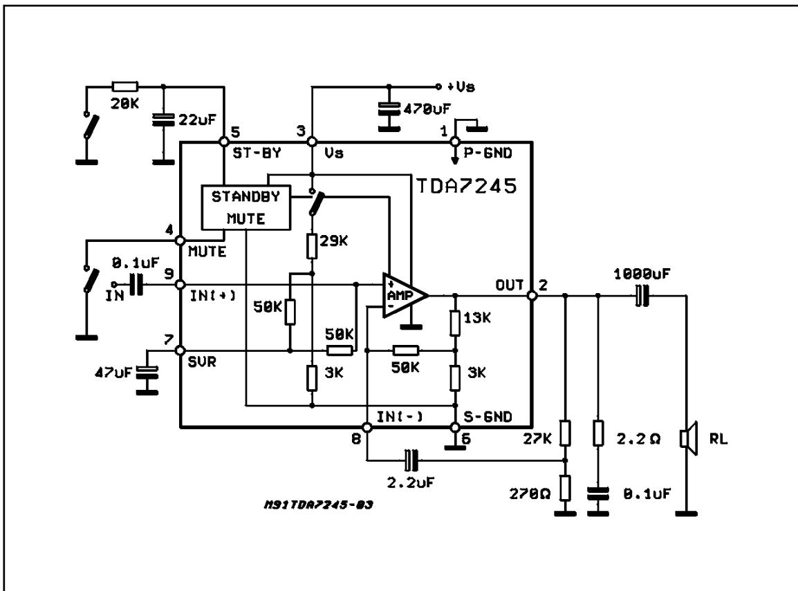
Figure 2: Schematic Diagram
