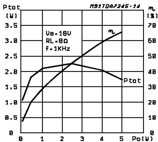
Figure 14: Power Dissipation & Efficiency vs. Output Power
