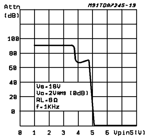
Figure 19: Output Attenuation vs. V_{pin5}
