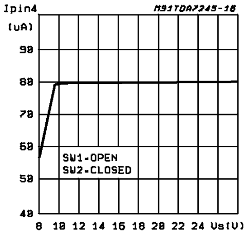
Figure 18: Quiescent Current (St-By) vs. Supply Voltage
