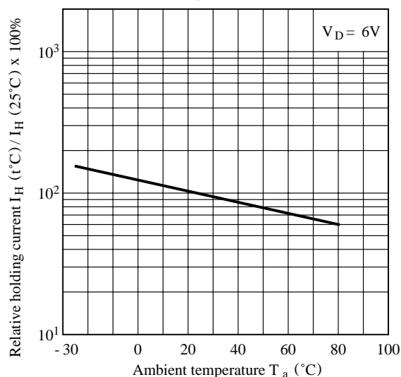
Fig. 7 Relative Holding Current vs. Ambient Temperature
