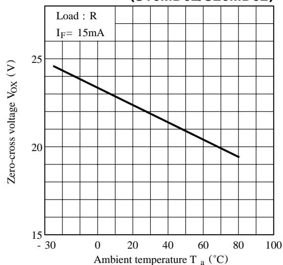
Fig.12 Zero-cross Voltage vs. Ambient Temperature (S16MD02/S26MD02)
