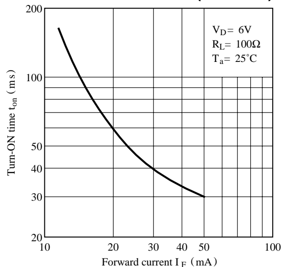
Fig.10 Turn-on Time vs. Forward Current (S26MD01)
