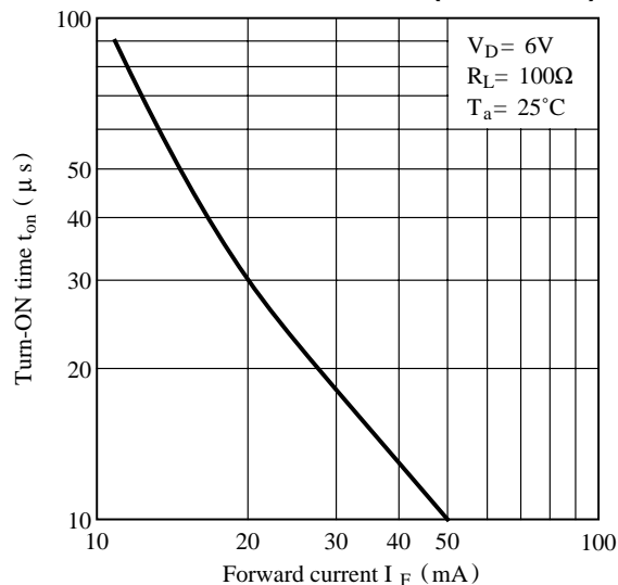
Fig. 9 Turn-on Time vs. Forward Current (S16MD01)
