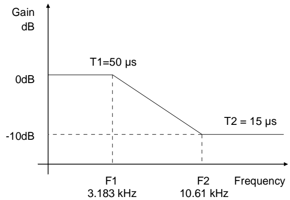
Figure 28. De-Emphasis Curve
