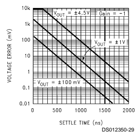
Voltage Error vs. Settle Time
