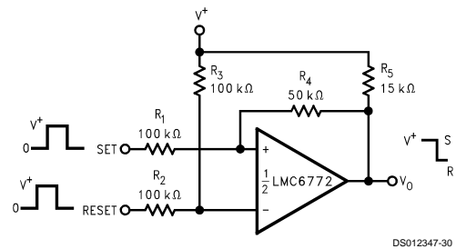
FIGURE 6. Bi-Stable Multivibrator
