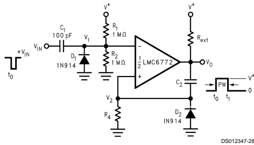
FIGURE 5. One-Shot Multivibrator
