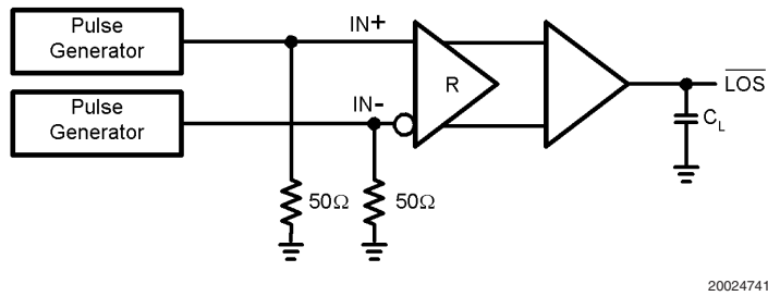
FIGURE 8. \overline{\text{LOS}} Output Load for Propagation Delay, and Rise/Fall Times
