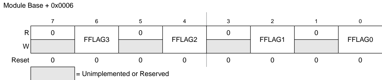
Figure 11-10. PMF Fault Flag Register (PMFFSTA)
