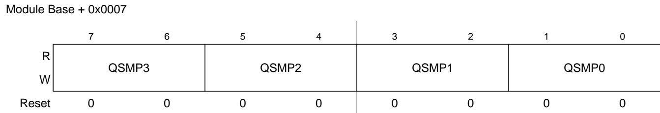
Figure 11-11. PMF Fault Qualifying Samples Register (PMFQSMP)
