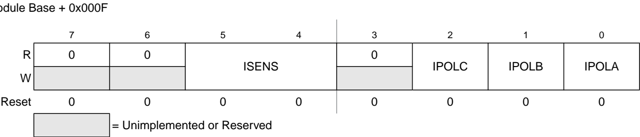
Figure 11-19. PMF Correction Control Register (PMFCCTL)
