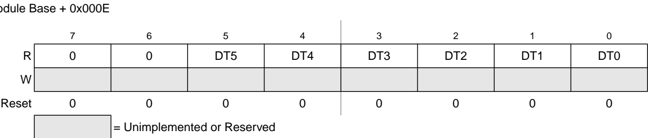
Figure 11-18. PMF Deadtime Sample Register (PMFDTMS))
