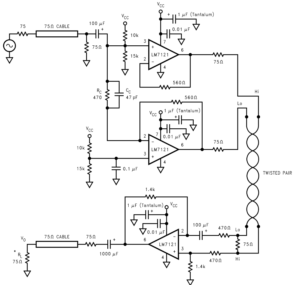
FIGURE 4. Single Supply Differential Twister Pair Cable Transmitter/Receiver 8.5V \leq V_{CC} \leq 30V
