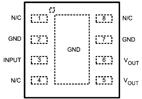
(Top View) Order Part Number LM3940LD-3.3 NSC Drawing Number LDC08A
