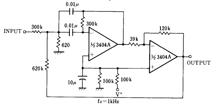
Bandpass Filter
