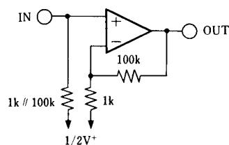
Test Circuit (Voltage Gain/Phase)
