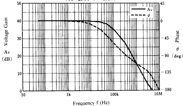
Voltage Gain/Phase vs. Frequency
