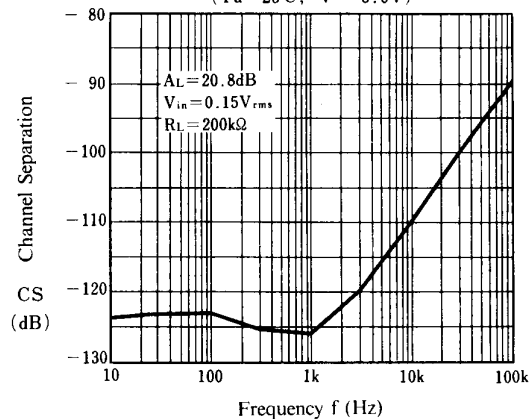
Channel Separation vs. Frequency
