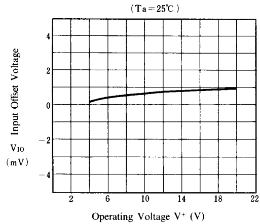
Input Offset Voltage vs. Operating Voltage
