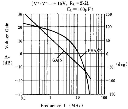
Voltage Gain, Phase vs. Frequency
