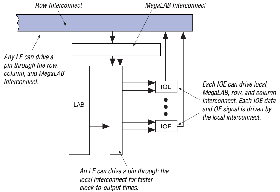
Figure 26. Row IOE Connection to the Interconnect
