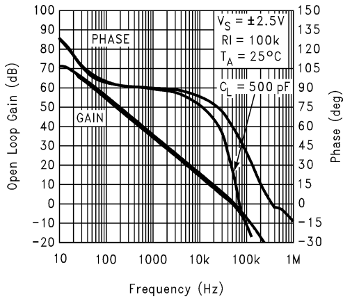
Gain and Phase vs. Capacitive Load @ 5V
