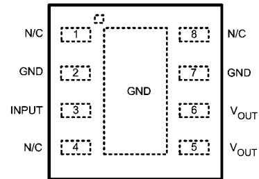
Top View See NS Package Number LDC08A
