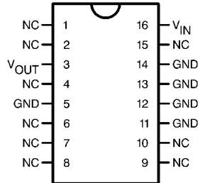
Top View See NS Package Number J16A
