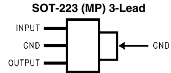
Front View See NS Package Number MP04A
