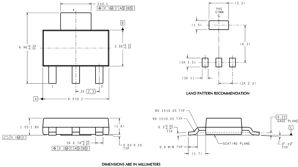
DIMENSIONS ARE IN MILLIMETERS
