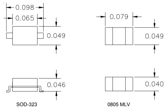
SOD-323
