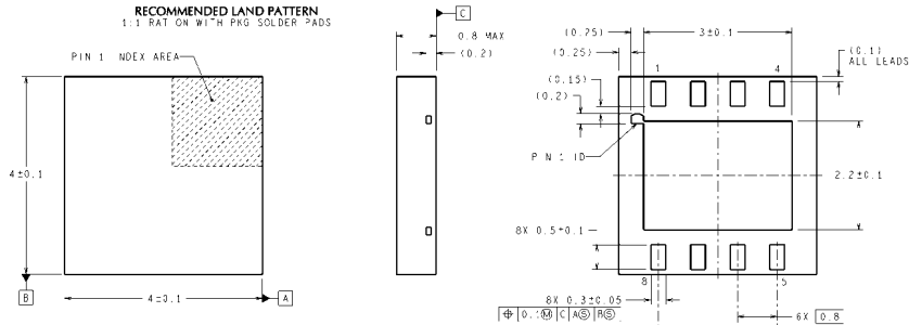
8-Lead LLP Order Number LM2940LD-5.0, LM2940LD-8.0, LM2940LD-9.0, LM2940LD-10, LM2940LD-12 or LM2940LD-15 NS Package Number LDC08A
