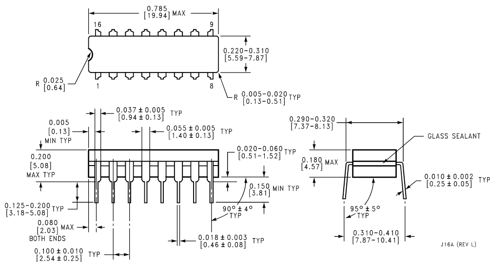
16-Lead Ceramic Dual-in-Line Package (J) Order Number LM2595J-3.3-QML (5962-9687901QEA), LM2595J-5.0-QML (5962-9650301QEA), LM2595J-12-QML (5962-9650201QEA), or LM2595J-ADJ-QML (5962-9650401QEA) NS Package Number J16A
