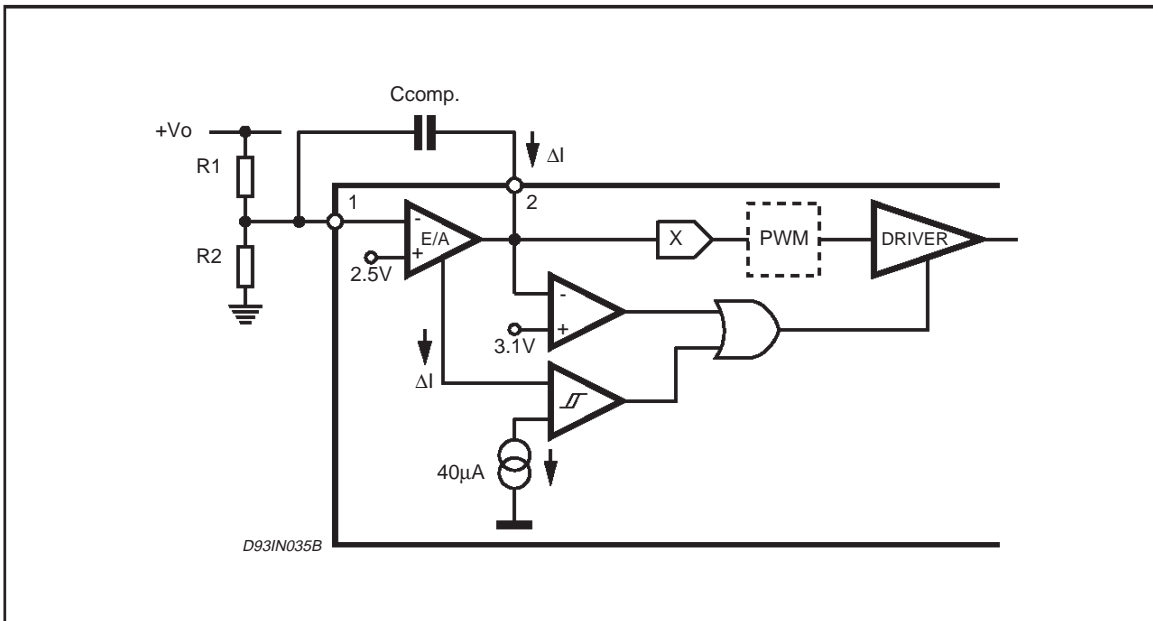
Figure 2: Overvoltage Protection Circuit
