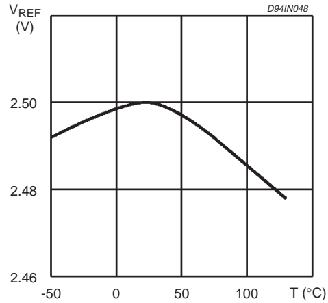
Figure 9: Voltage Feedback Input Threshold vs. Temperature
