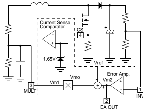
Fig.3.1 Multiplier Block
