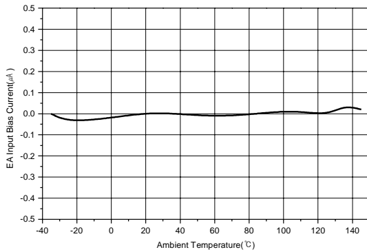
Figure 10. EA Input Bias Current vs Temperature
