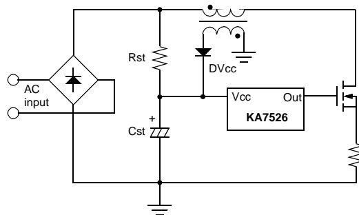
Fig.1.1 Start-up Circuit
