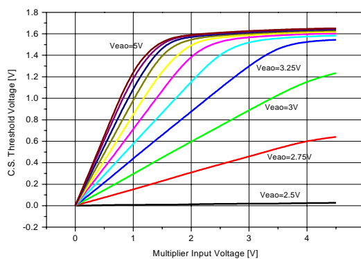
Figure 2. Multiplier Input Voltage vs C.S. Threshold
