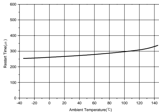
Figure 14. Restart Time vs Temperature
