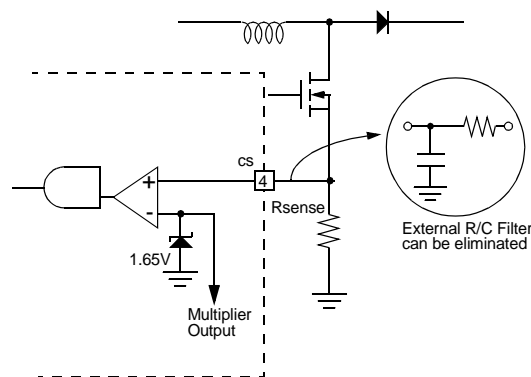
Fig. 4.1 Current Sense Circuit
