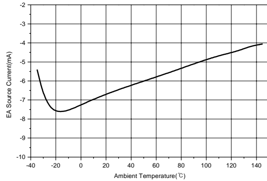
Figure 8. EA Source Current vs Temperature
