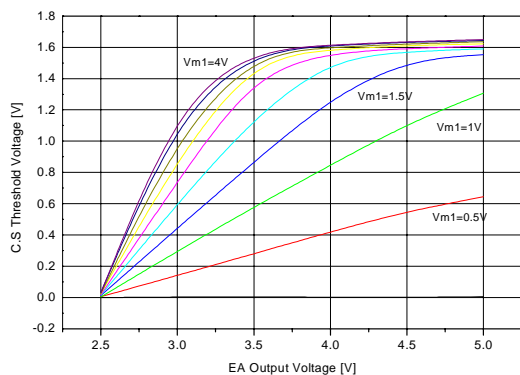
Figure 1. EA Output Voltage vs C.S. Threshold
