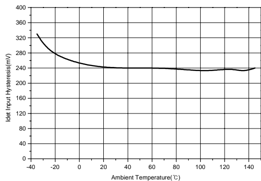
Figure 13. Idet Input Hysteresis vs Temperature
