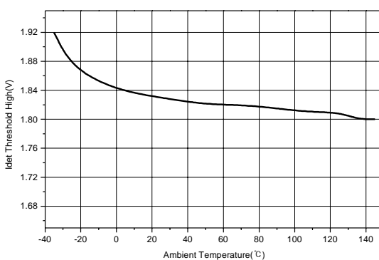
Figure 12. Idet Threshold Voltage vs Temperature
