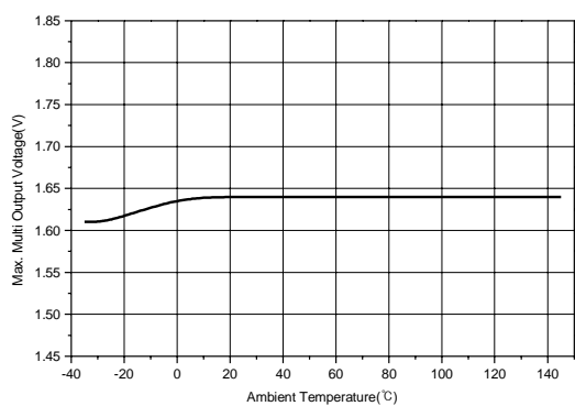
Figure 15. Max.Mult.Output Voltage vs Temperature
