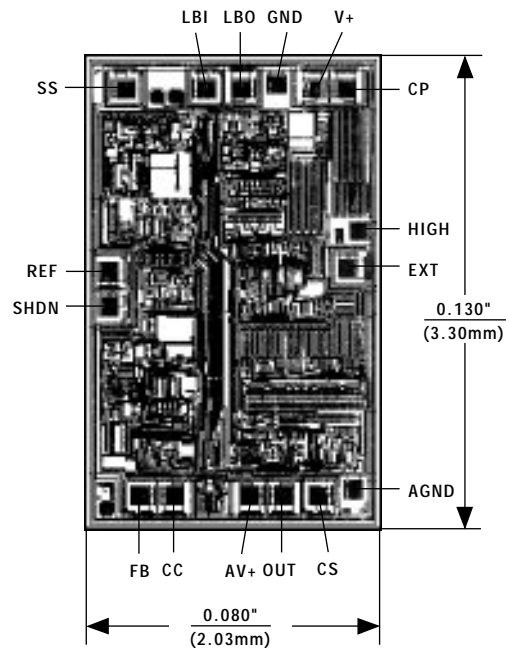
Chip Topography
