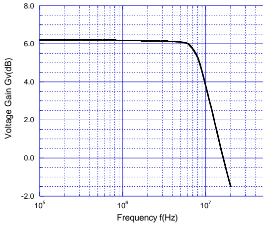
Voltage Gain vs. Frequency
