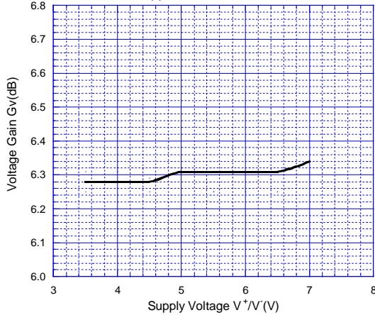
Voltage Gain vs. Supply Voltage
