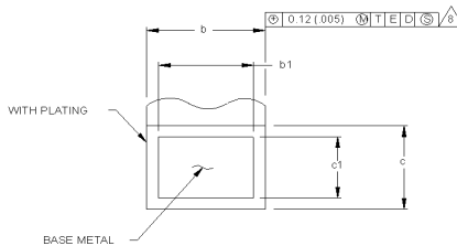
DETAIL "C" (SEE NOTE 9)
