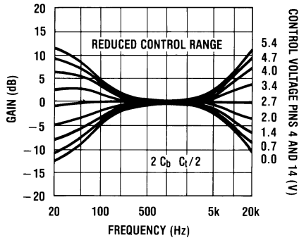
FIGURE 4. Tone Characteristic (Gain vs Frequency)
