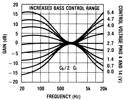
FIGURE 5. Tone Characteristic (Gain vs Frequency)
