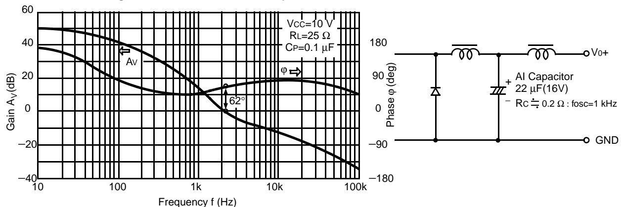
Fig. 33 - DC/DC Converter +5 V output
