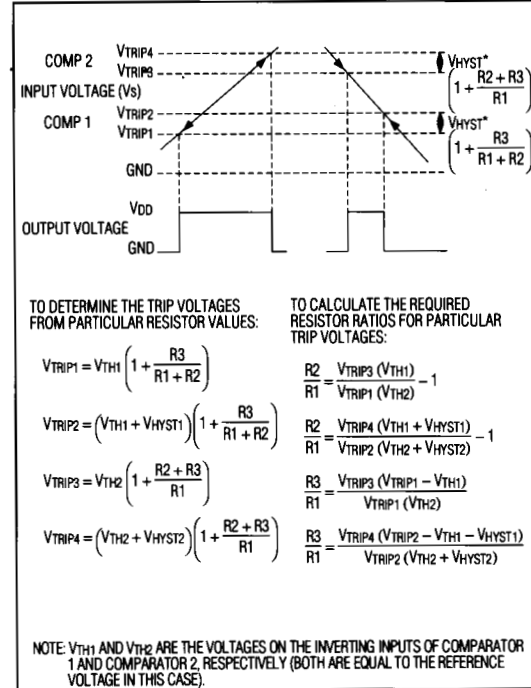
Figure 12. Window Detector Waveforms and Formulas
