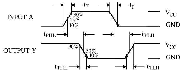
Figure 1. Switching Waveforms
