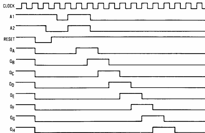
Figure 3. Switching Waveforms
