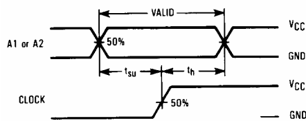
Figure 3. Switching Waveforms
