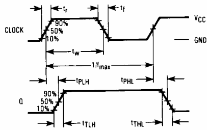
Figure 1. Switching Waveforms
