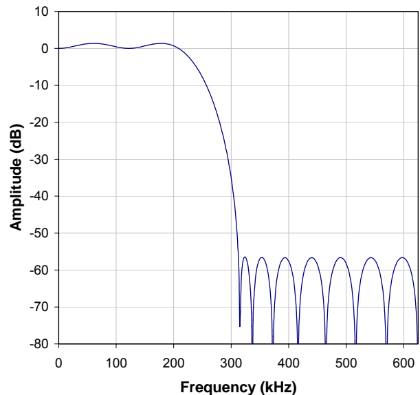
Figure 20. 24-Tap FIR Frequency Response
