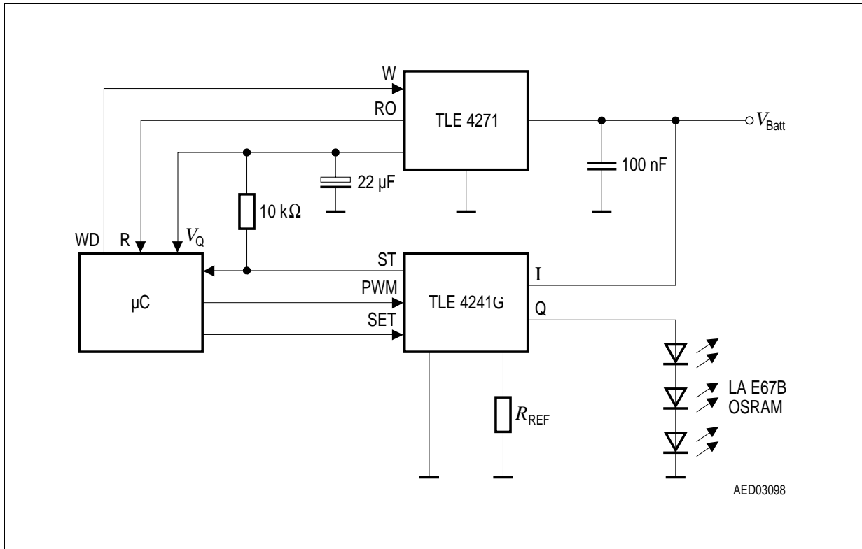
Figure 3 Application Circuit
