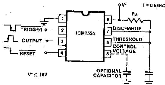
Figure 4: Monostable Operation
