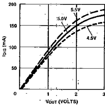
COMMON CATHODE DIGIT DRIVER
