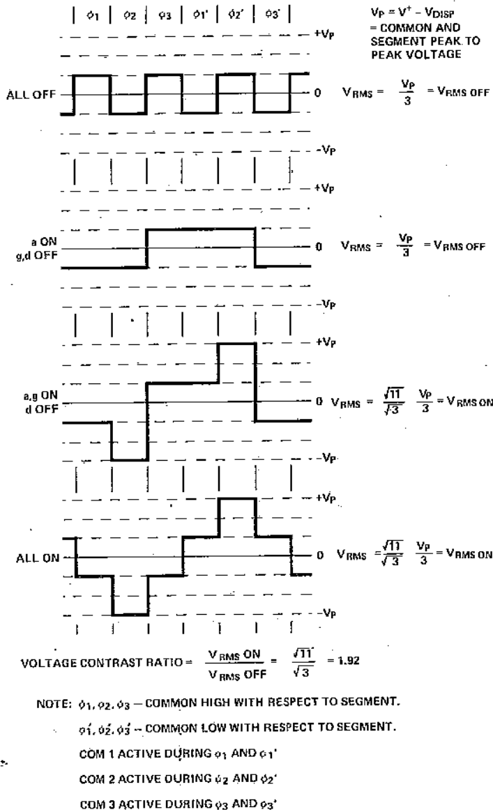
Figure 4. Voltage Waveforms on Segment g ( V_g )
