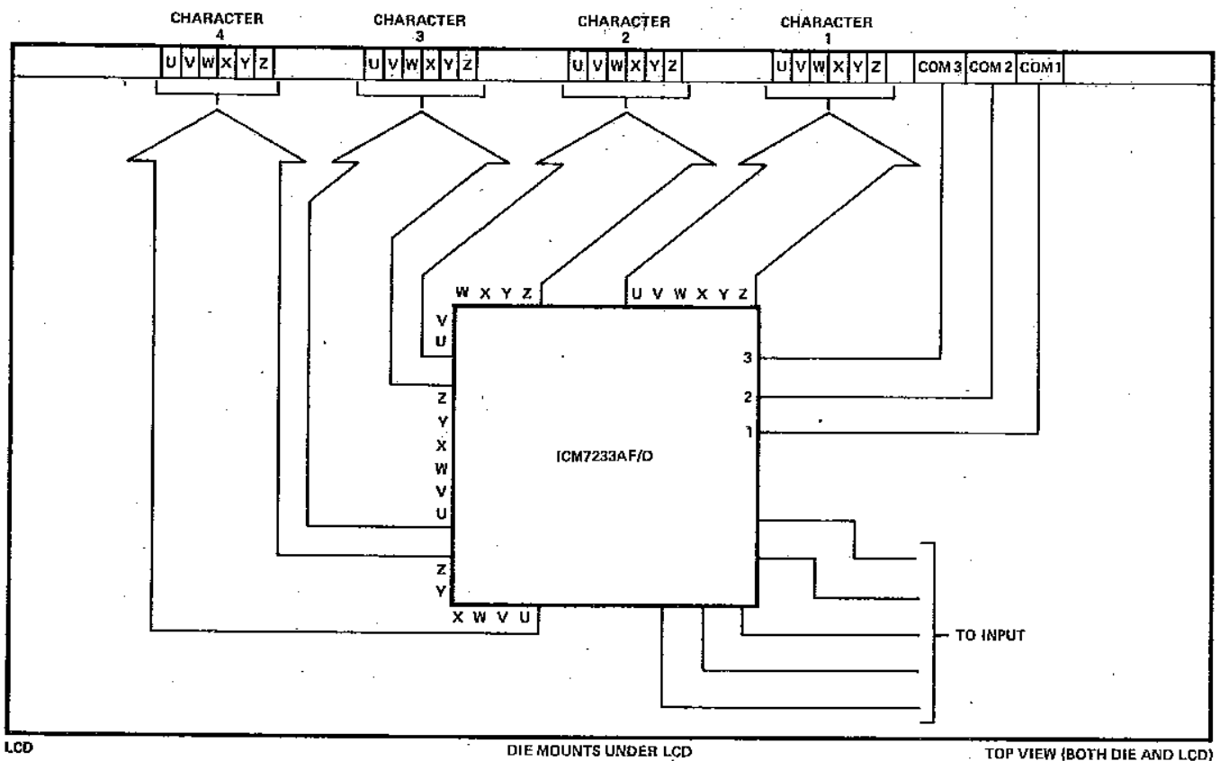
Figure 27. "Forward" Die Pad Orientation and Typical Triplet Alphanumeric Display Orientation
