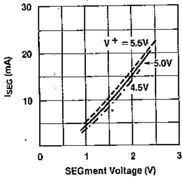
SEGment Current vs Output Voltage
