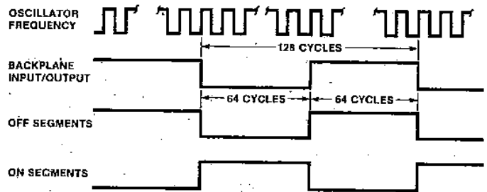
Display Waveforms
