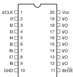
DIP/SOIC
