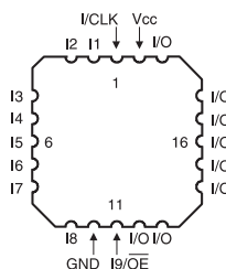
PLCC Top View
