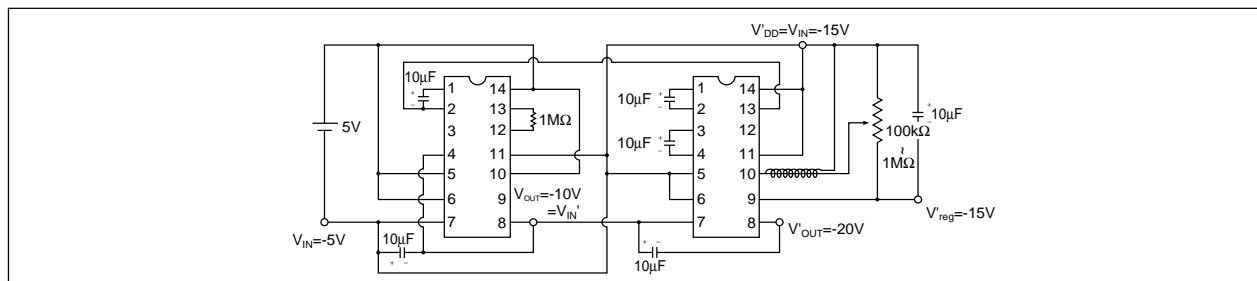
Serial Connection
