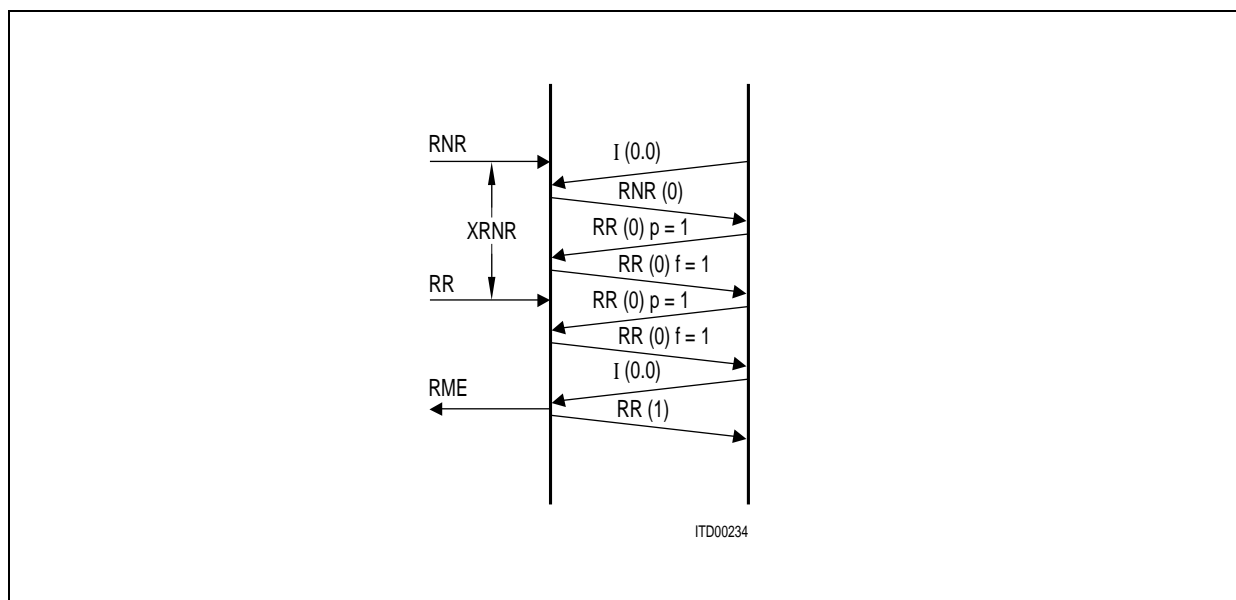
Figure 13 Flow Control/Reception
