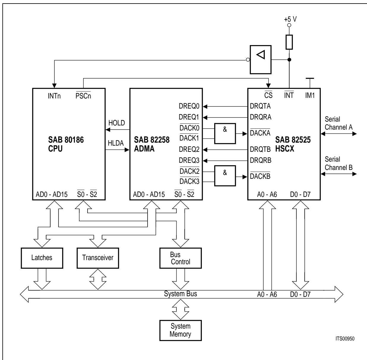
Figure 5 HSCX with SAB 80186 CPU/SAB 82258 ADMA
