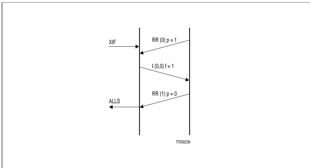
Figure 18 Data Transmission (no Error)
