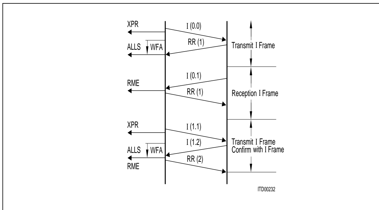
Figure 12 Transmission/Reception I-Frames
