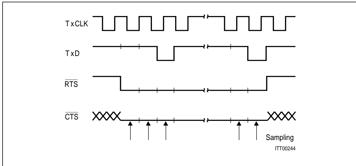
Figure 31 RTS-CTS Handshaking
