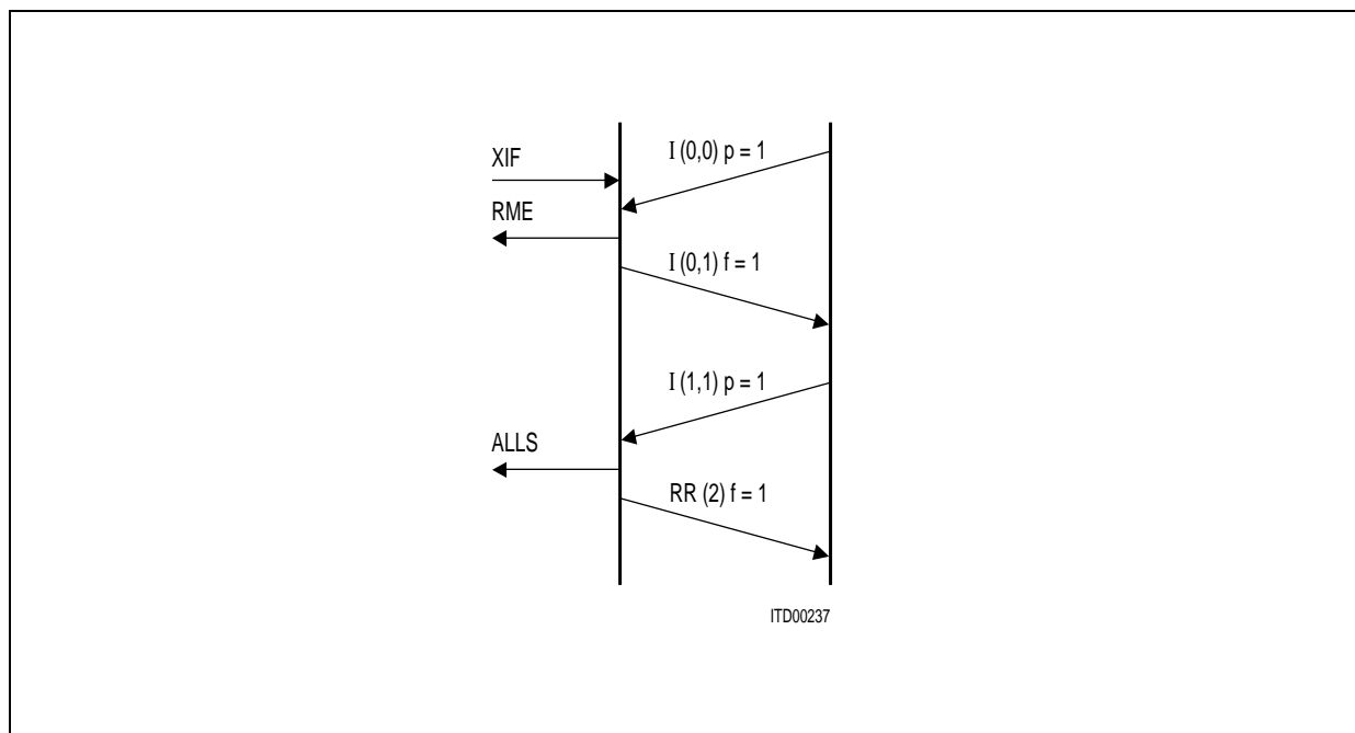
Figure 17 Data Reception/Transmission
