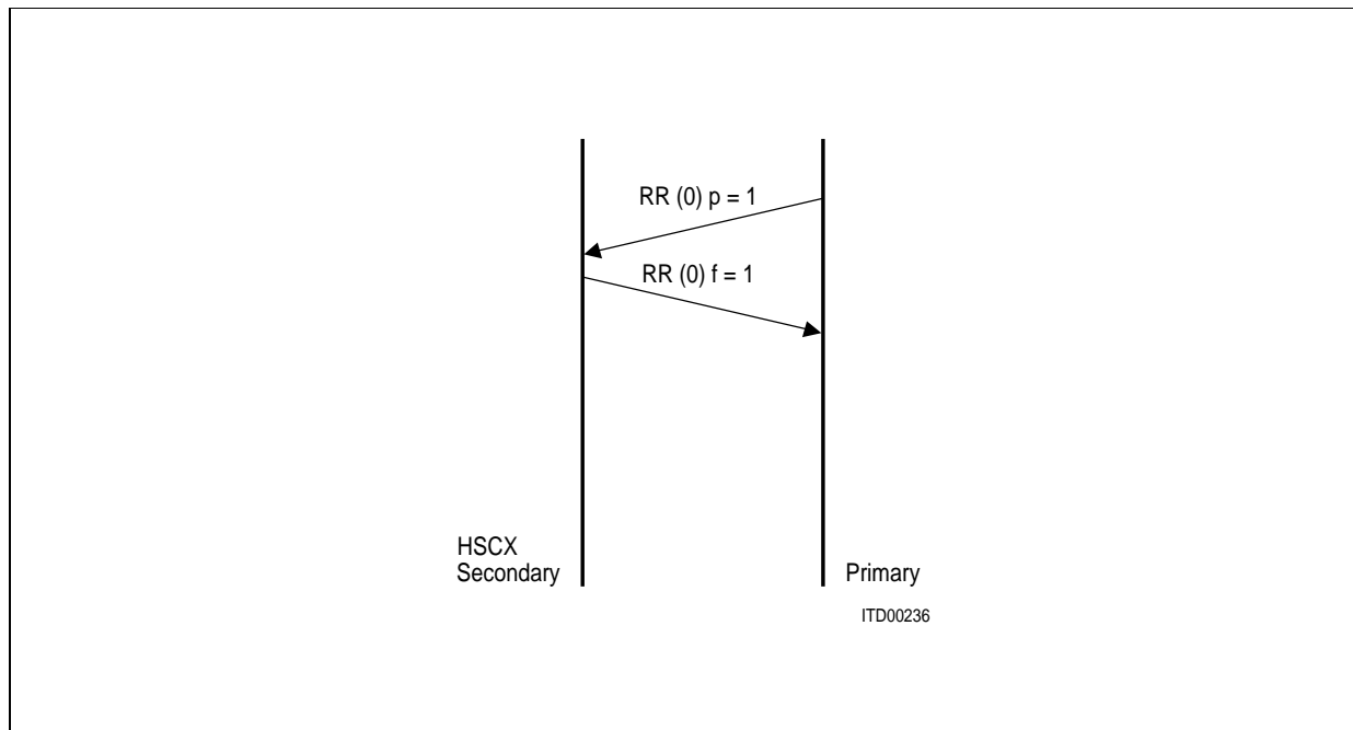
Figure 16 No Data to Send
