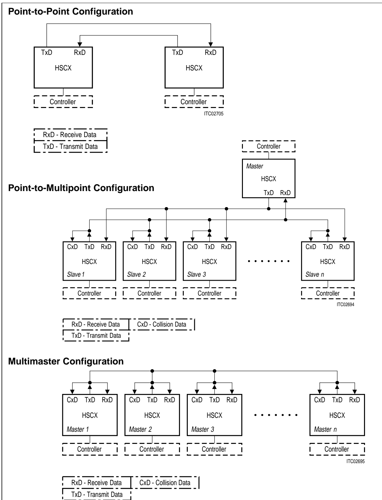
Figure 6 Link Configuration
