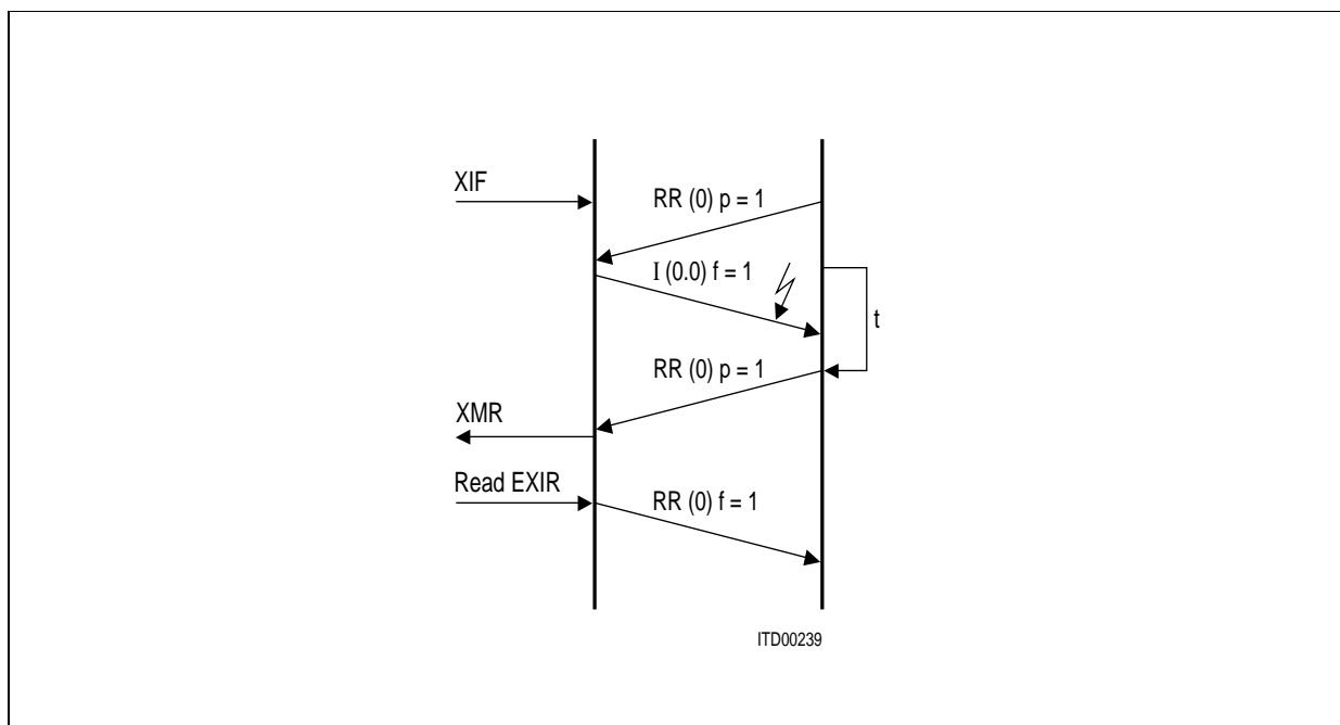
Figure 19 Data Transmission (Error)
