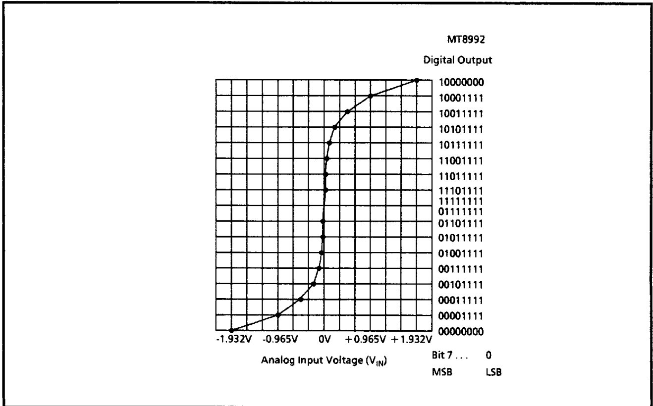
Figure 16 - μ-Law Encoder Transfer Characteristic
