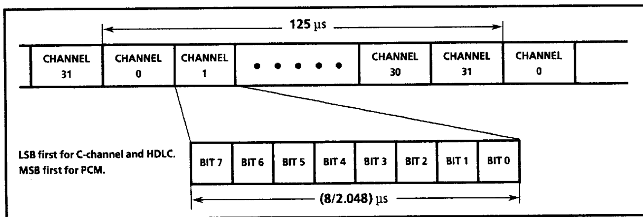
Figure 8 - Format of ST-BUS Stream
