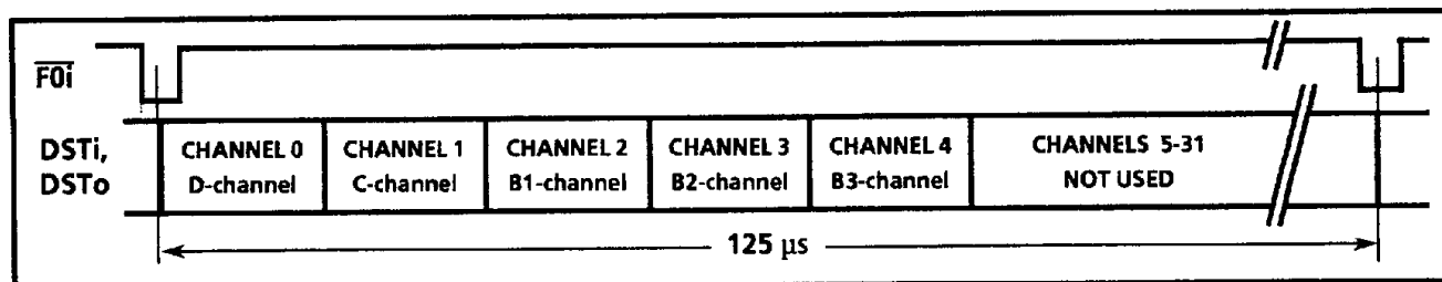
Figure 9 - DSTi and DSTo Channels Assignment
