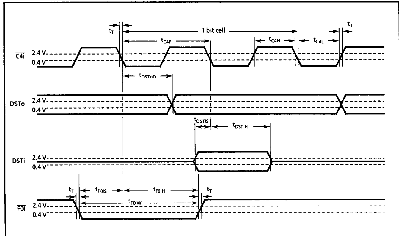
Figure 12 - ST-BUS Timing Diagram
