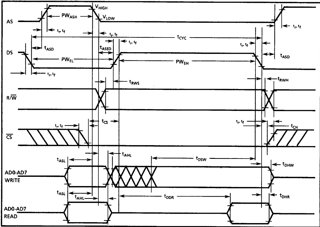
Figure 13 - Motorola BUS Timing
