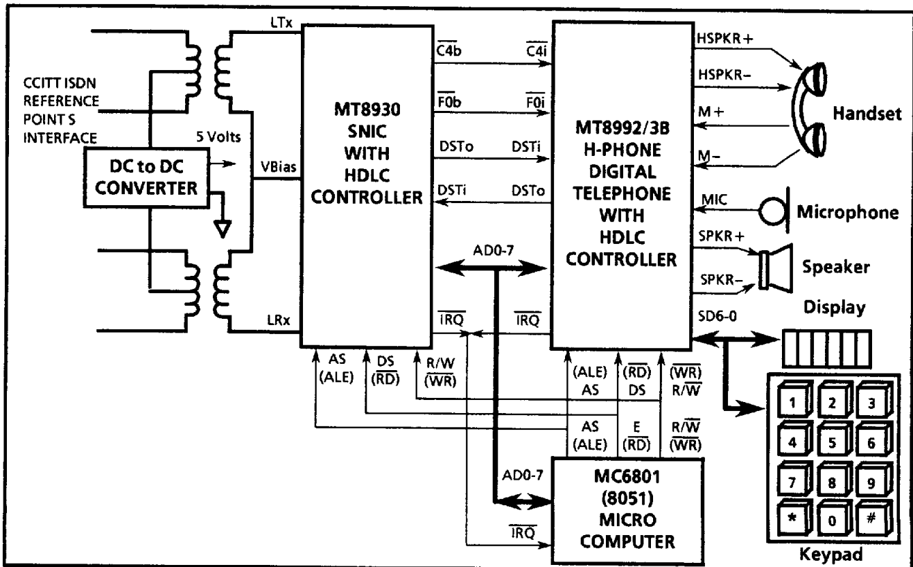
Figure 10 - CCITT ISDN Voice/Data Terminal Equipment - TE1
