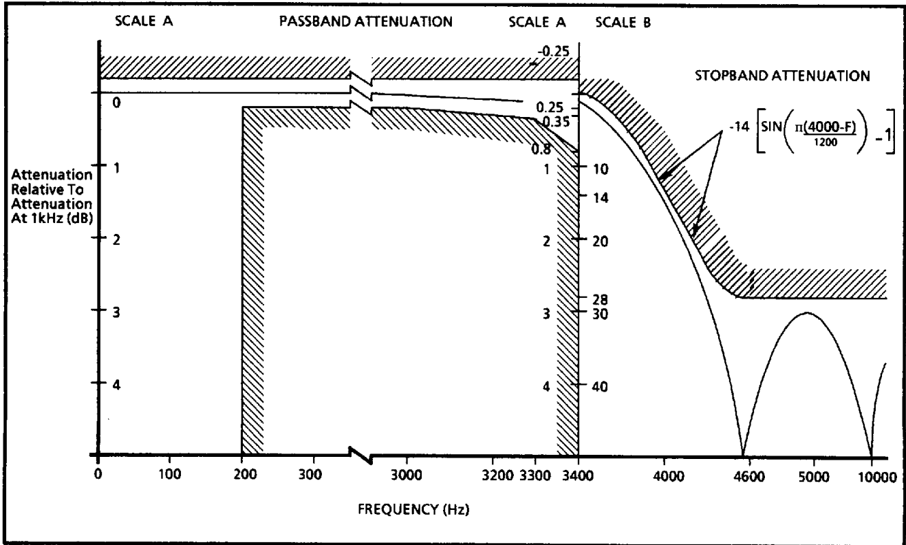
Figure 19 - Attenuation vs Frequency for Receive Filter
