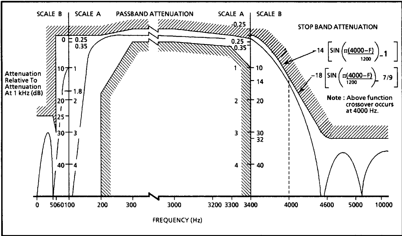
Figure 18 - Attenuation vs Frequency for Transmit Filter
