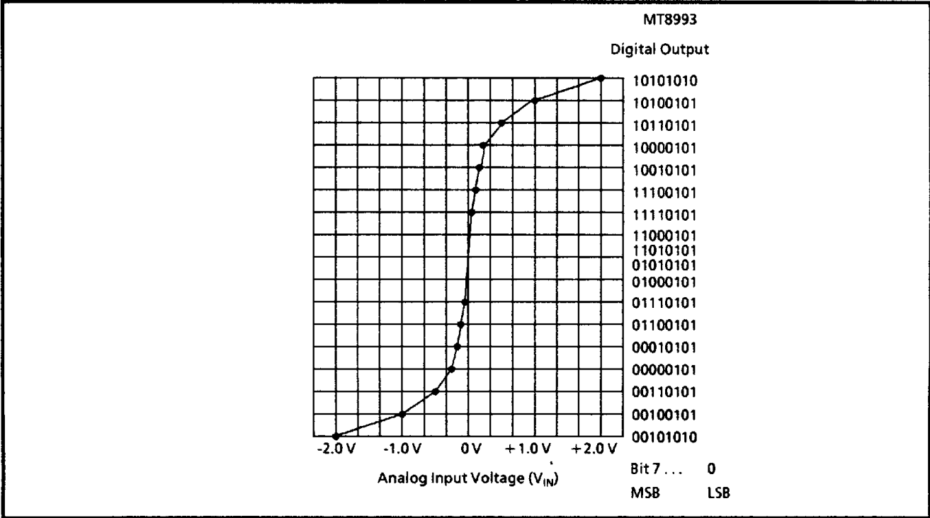
Figure 17 - A-Law Encoder Transfer Characteristic
