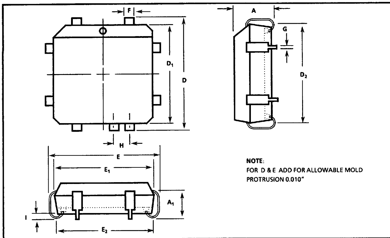
Plastic J-Lead Chip Carrier (P-Suffix)
