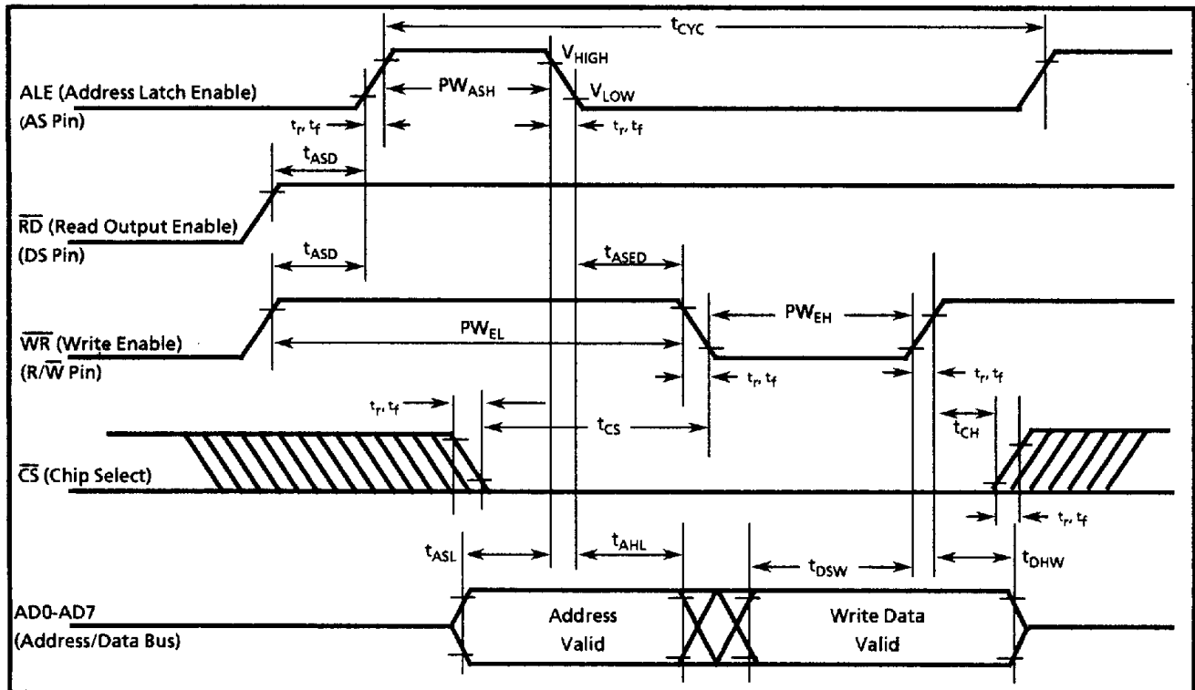
Figure 15 - Bus Write Timing Intel Multiplexed Bus
