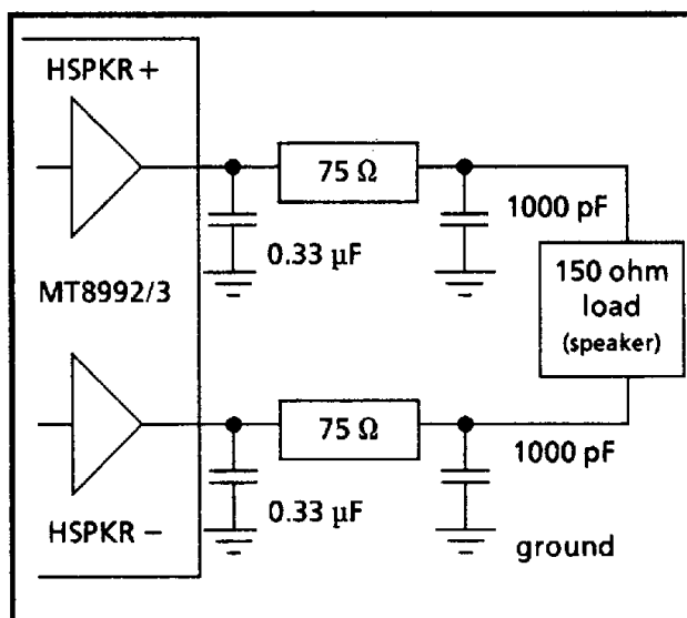
Figure 4 - Handset Speaker Driver
