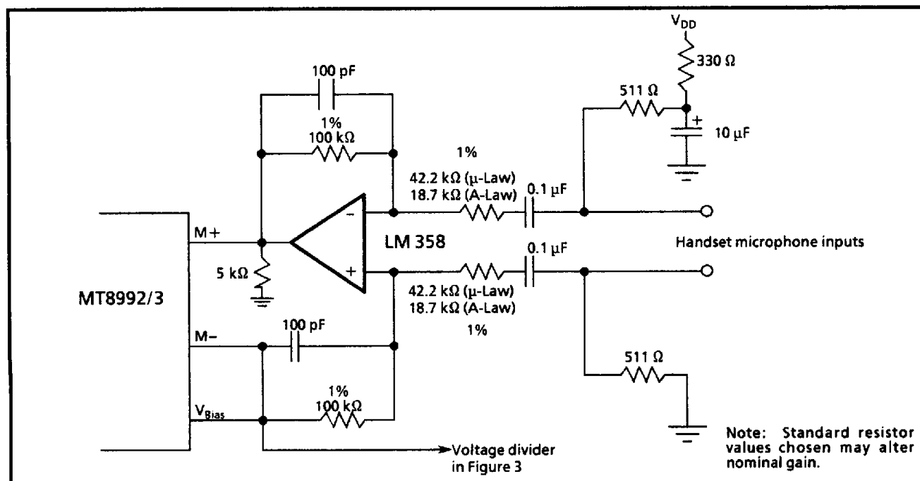
Figure 5 - Recommended Handset Microphone Interface Circuit
