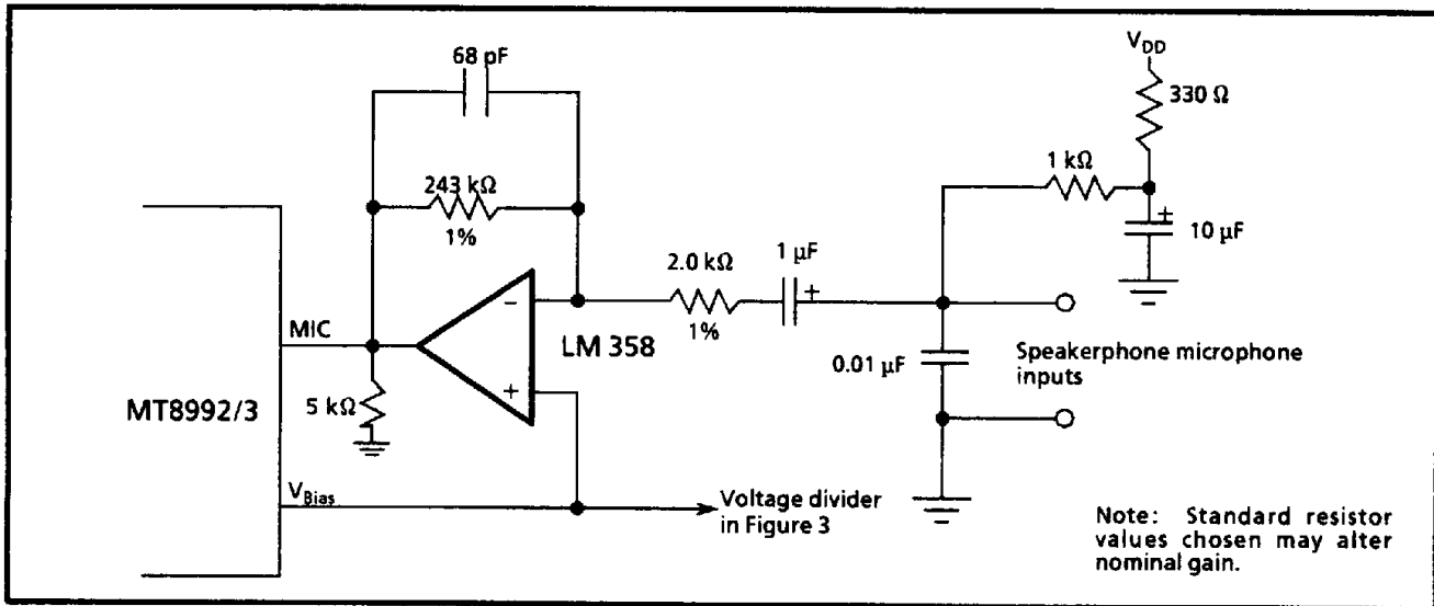
Figure 6 - Recommended Speakerphone Microphone Interface Circuit
