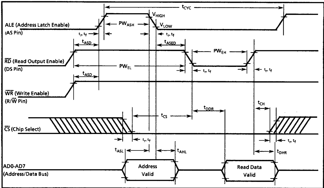
Figure 14 - Bus Read Timing Intel Multiplexed Bus
