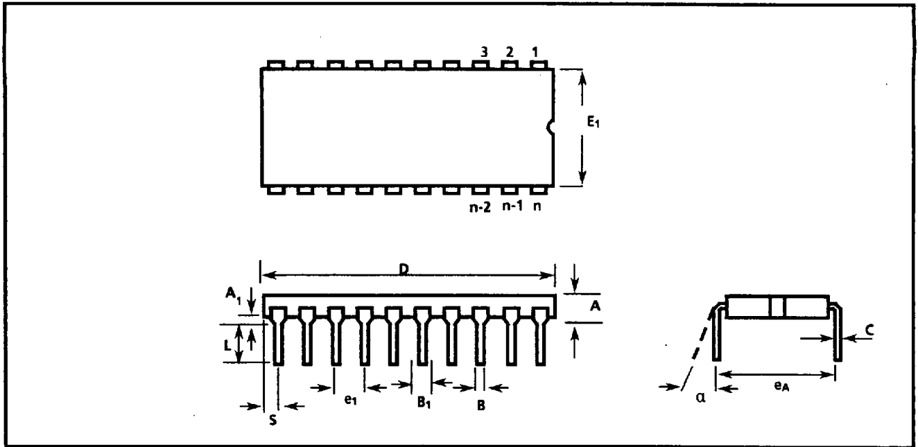
Ceramic Dual-In-Line Packages (CDIP) - C Suffix
