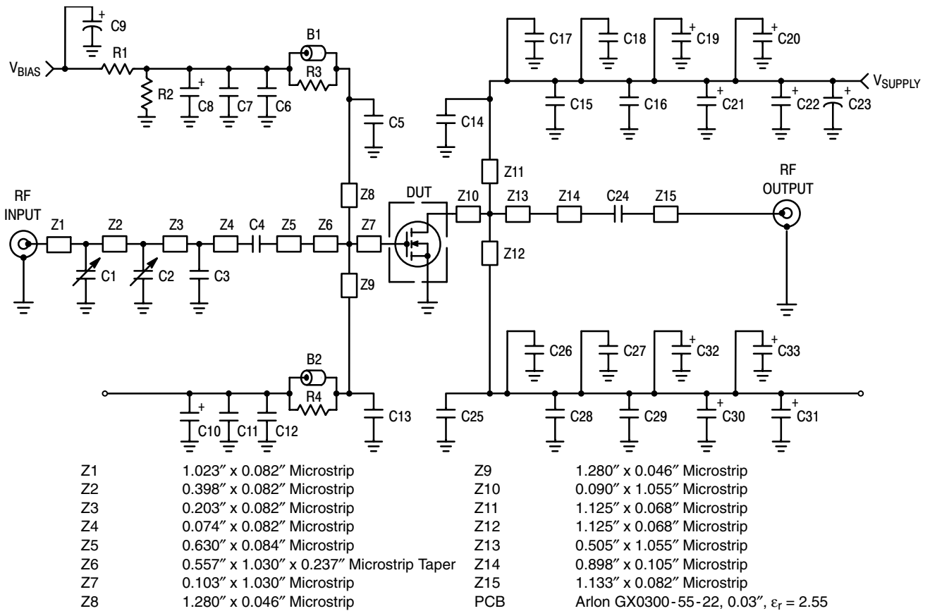
Figure 1. MRF5S19150HR3(SR3) Test Circuit Schematic
