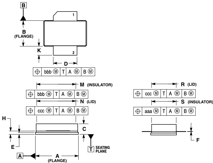
CASE 465C-02 ISSUE A NI-880S MRF5S19150HSR3
