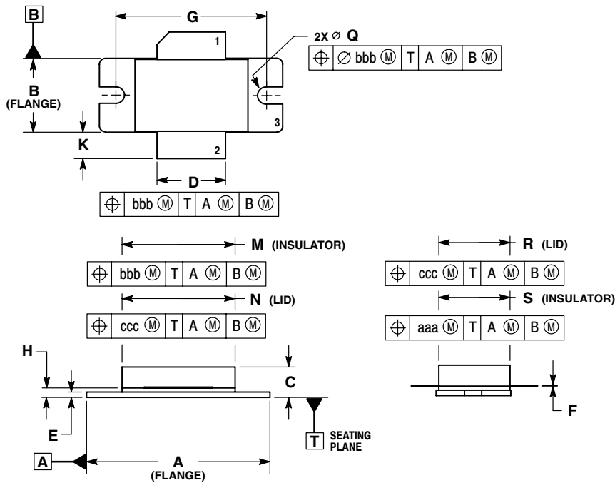
CASE 465B-03 ISSUE B NI-880 MRF5S19150HR3
