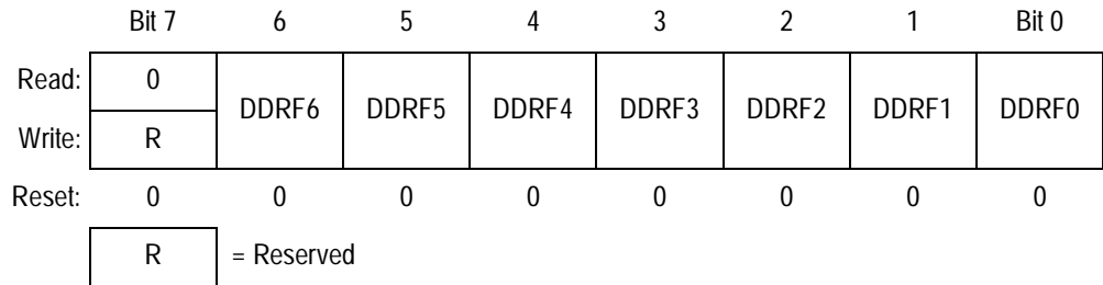
Figure 20-18. Data Direction Register F (DDRF)
