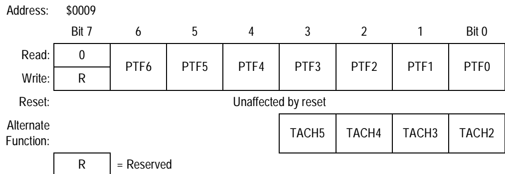
Figure 20-17. Port F Data Register (PTF)
