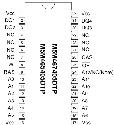
Outline 32P3N (400mil TSOP Normal Bend)
