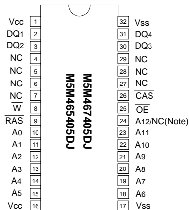
Outline 32P0N (400mil SOJ)
