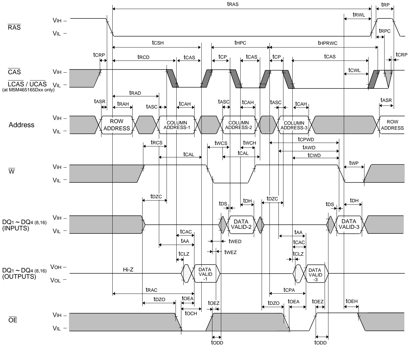
EDO Mode Mix Cycle (1) (Note 30)
