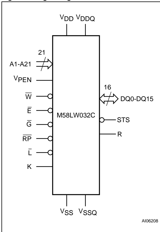
Figure 2. Logic Diagram
