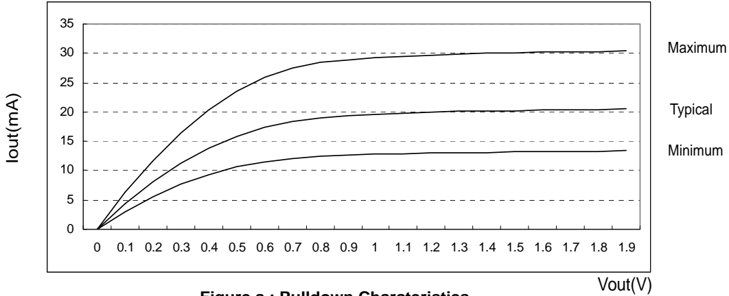
Figure a : Pulldown Charateristics
