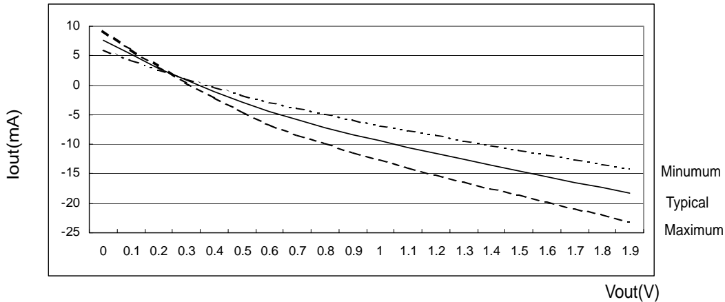
Figure b : PulluP Charateristics
