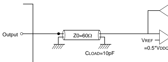
(Fig. 1) Output Load Circuit
