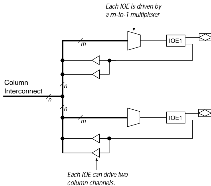
Figure 17. ACEX 1K Column-to-IOE Connections
