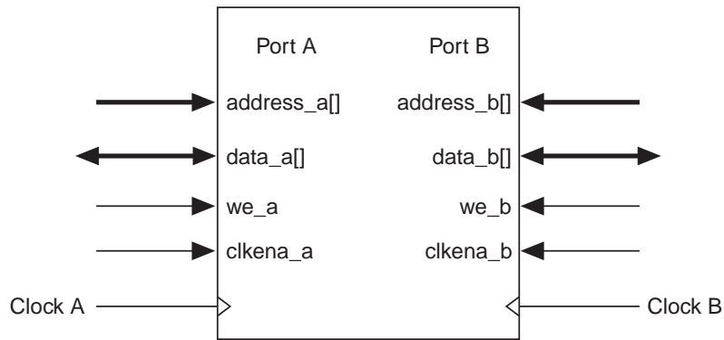
Figure 3. ACEX 1K EAB in Dual-Port RAM Mode
