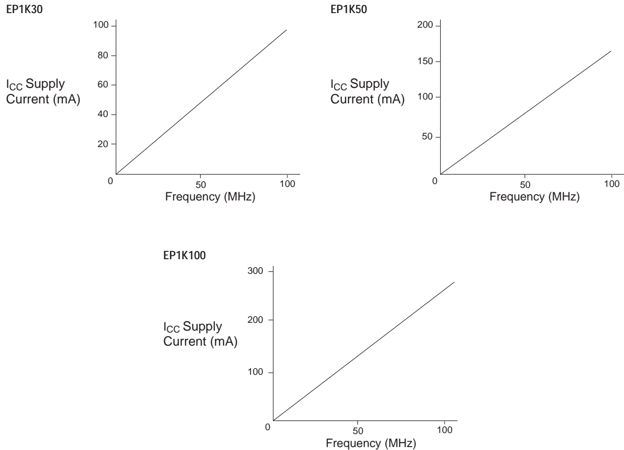
Figure 29. ACEX 1K I_{CCACTIVE} vs. Operating Frequency
