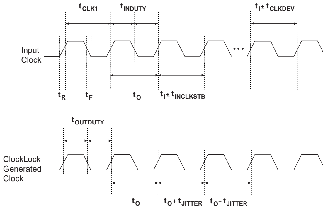
Figure 19. Specifications for the Incoming & Generated Clocks Note (1)
