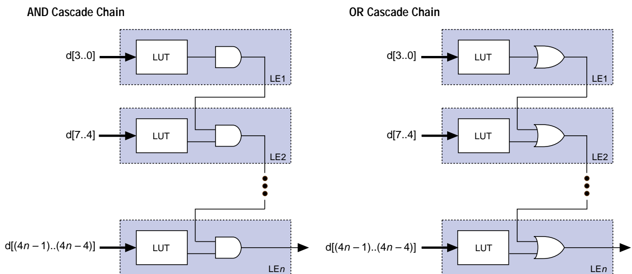
Figure 10. ACEX 1K Cascade Chain Operation
