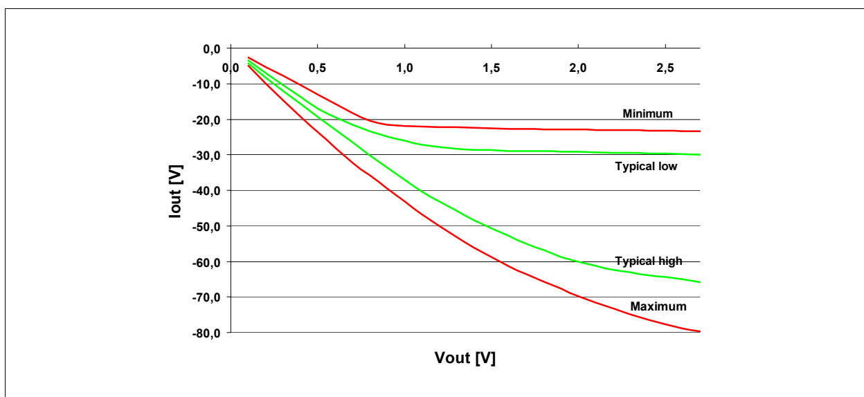
Figure 37 Weak Strength Pull-up Characteristics
