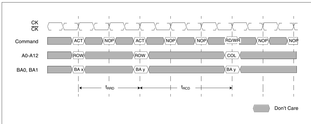
Figure 8 t_{\text{RCD}} and t_{\text{RRD}} Definition
