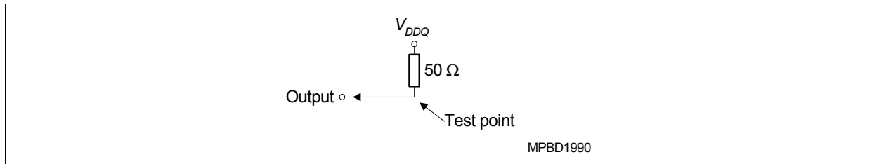
Figure 52 Pullup slew rate test load
