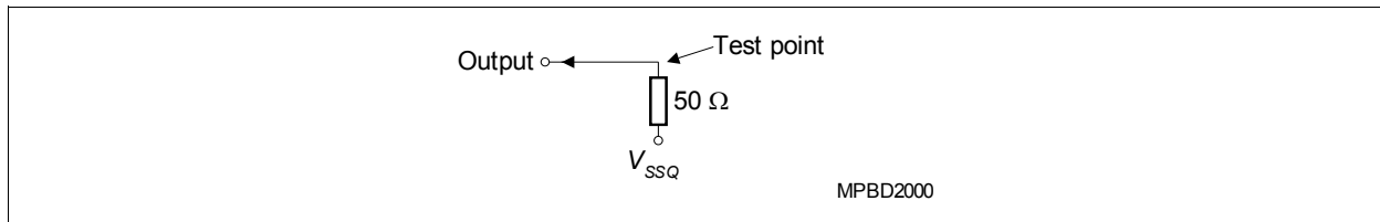
Figure 53 Pulldown slew rate test load
