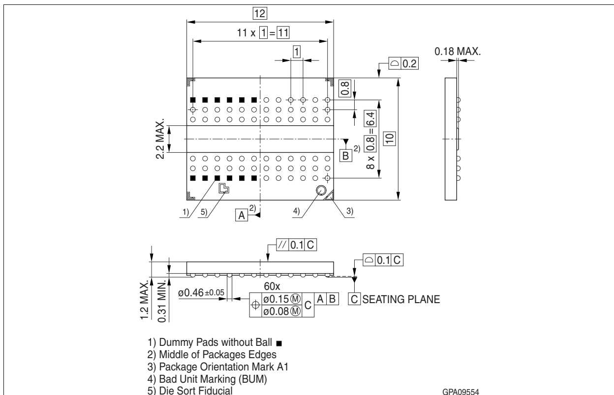
Figure 54 Package Outline of P-TFBGA-60-[9/22] (green/non-green)
