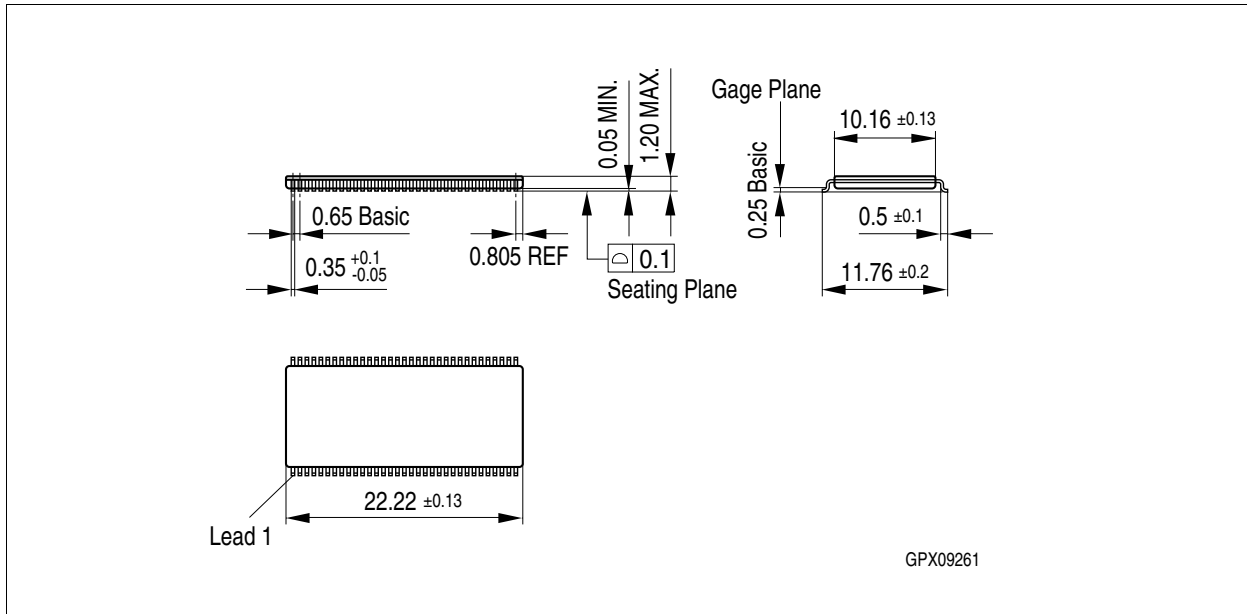
Figure 55 Package Outline of P-TSOPII-66-1 (green/non-green)
