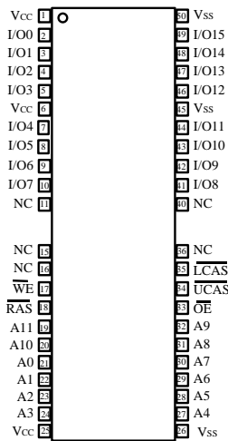
44(50) TSOP II
