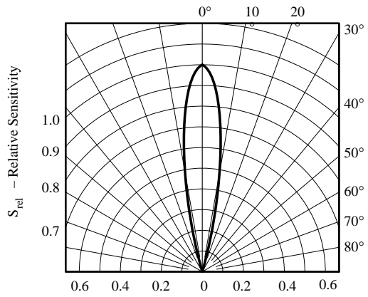
Figure 9. Relative Radiant Sensitivity vs. Angular Displacement
