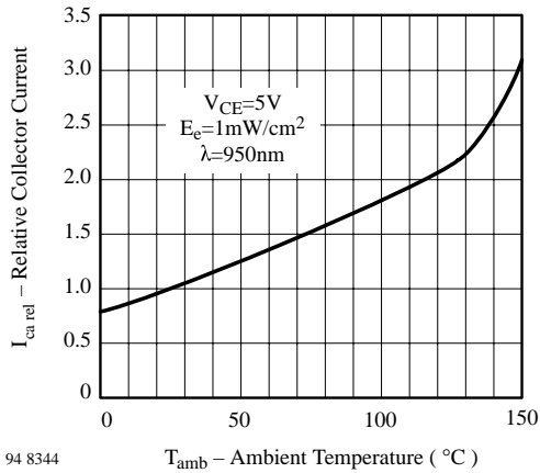
Figure 3. Relative Collector Current vs. Ambient Temperature
