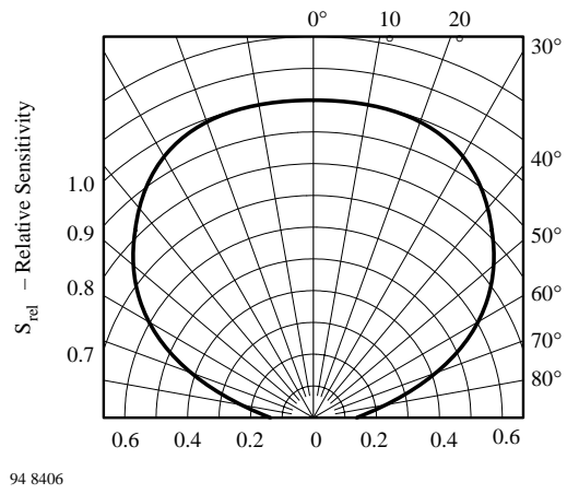
Figure 7. Relative Radiant Sensitivity vs. Angular Displacement
