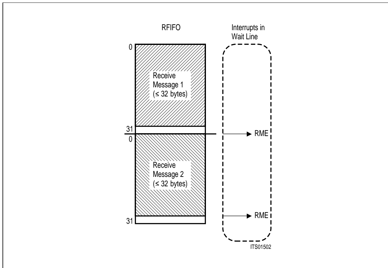
Figure 57 Contents of RFIFO (short message)
