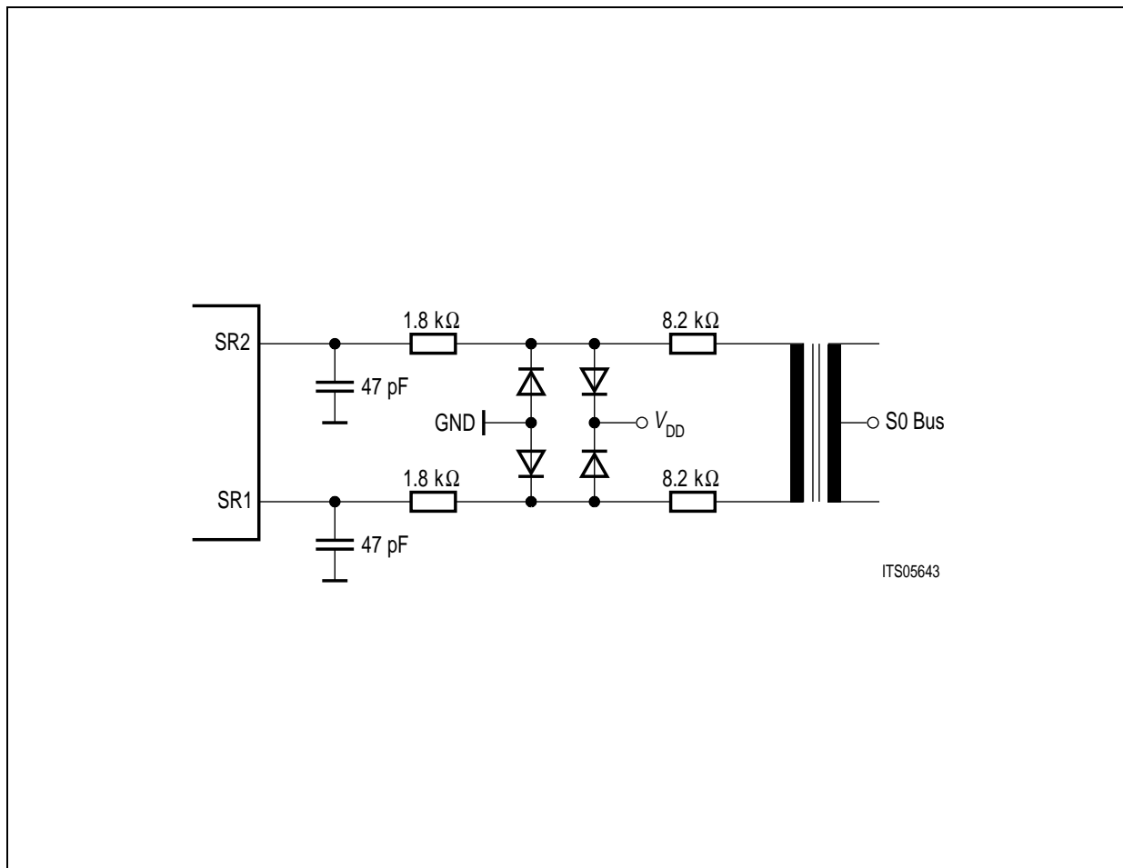
Figure 49 External Circuitry for Symmetrical Receivers
