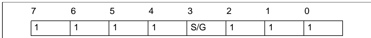
Figure 26 MONITOR Channel on IDP0
