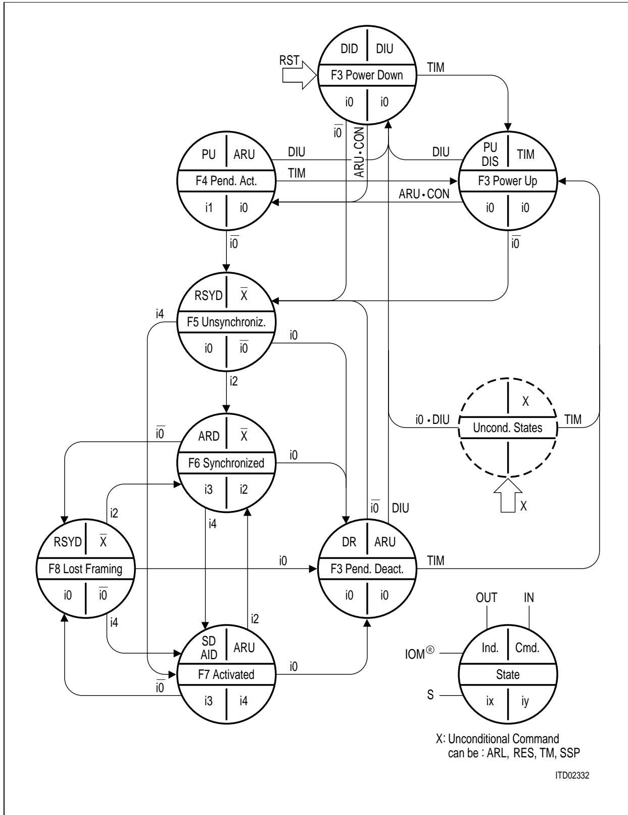
Figure 75a State Diagram of TE/LT-T Mode
