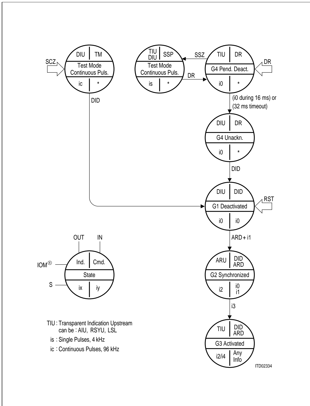
Figure 76 State Diagram of LT-S Mode
