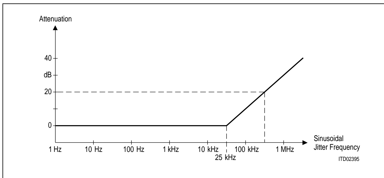
Figure 105 Jitter Transfer Curve of XPLL
