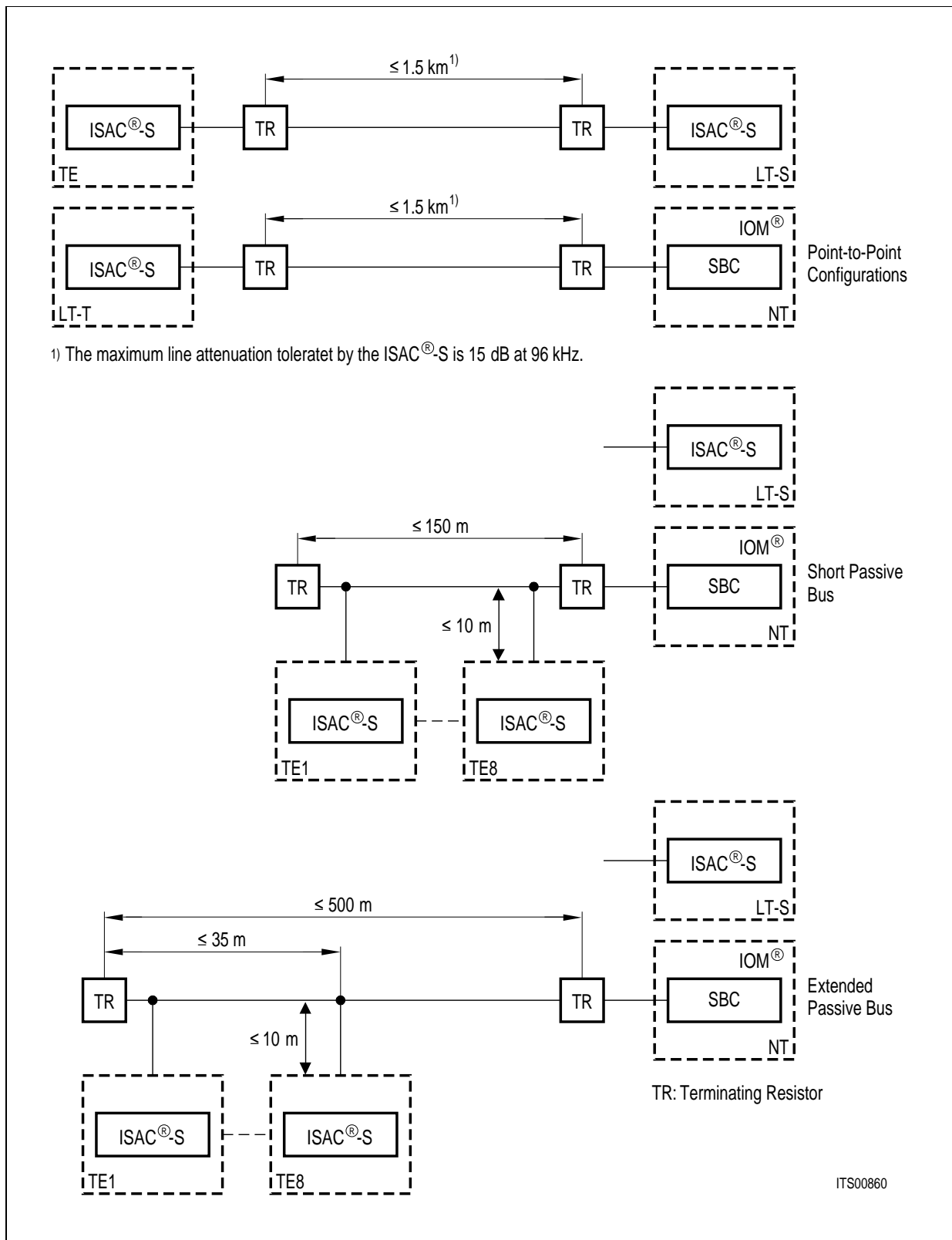
Figure 41 Wiring Configurations in User Premises
