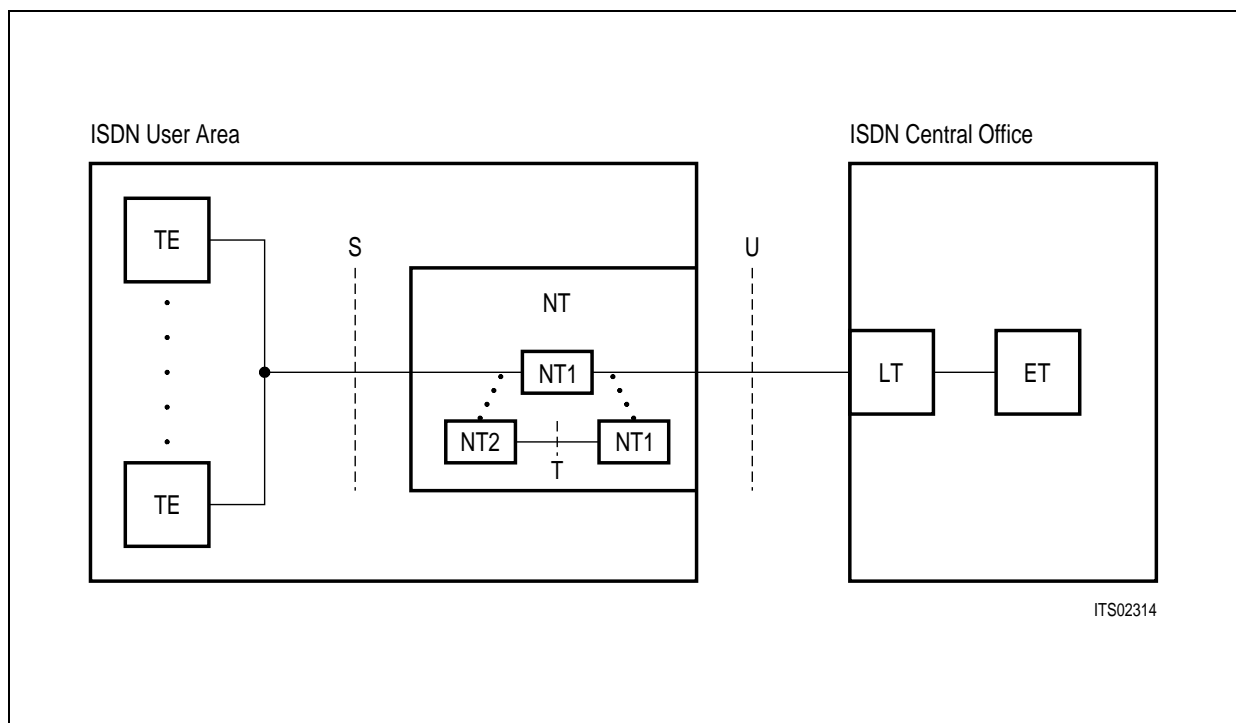
Figure 4 ISDN Basic Subscriber Access Architecture
