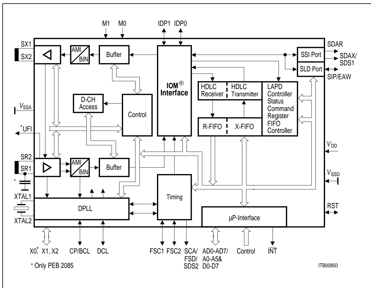
Figure 10 Architecture of the ISAC ® -S
