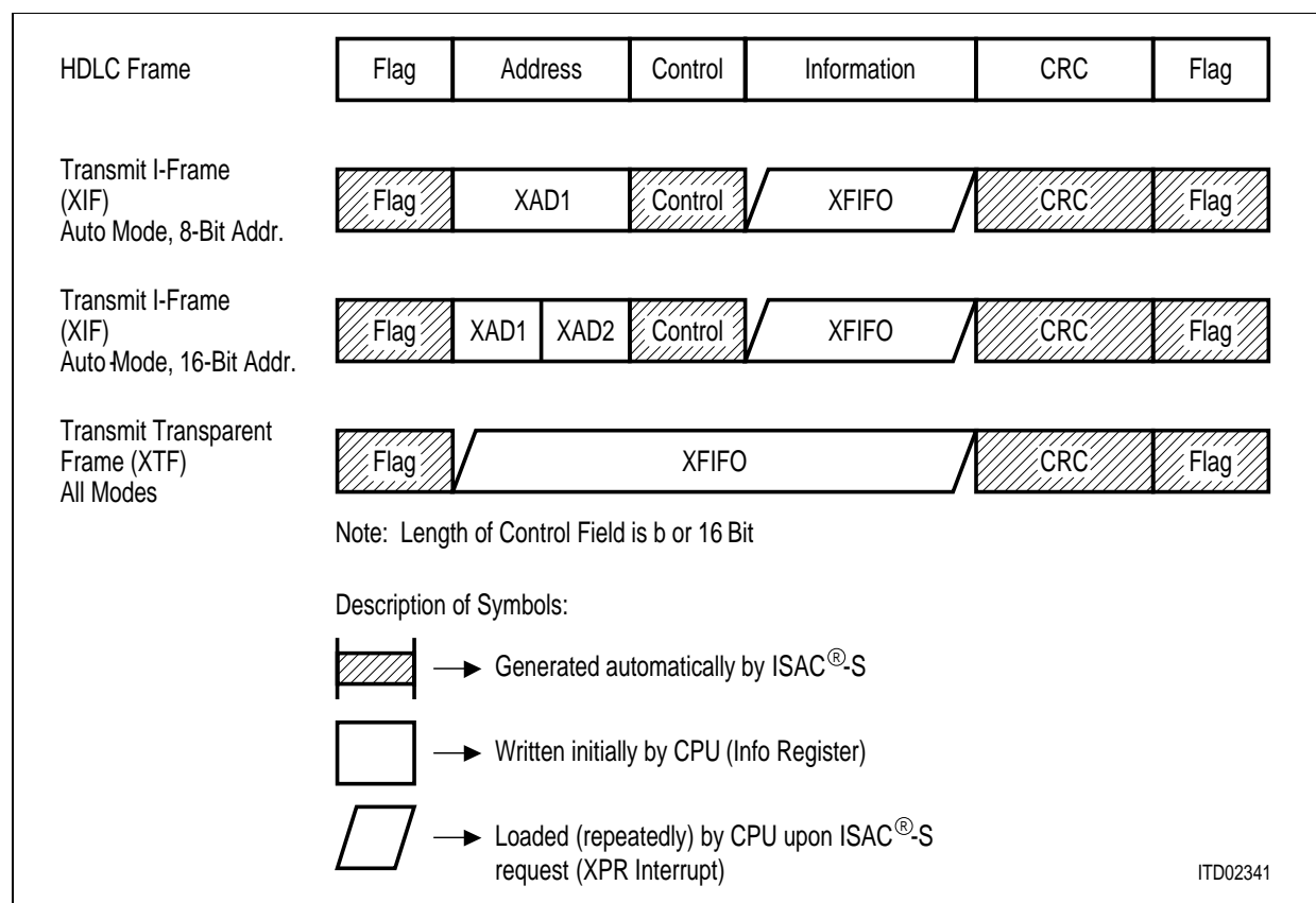
Figure 81 Transmit Data Flow
