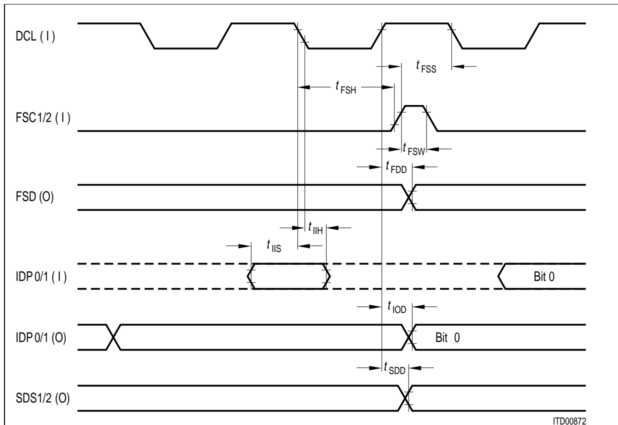
Figure 96 IOM® Timing (LT-S, LT-T, NT mode) IOM® Timing
