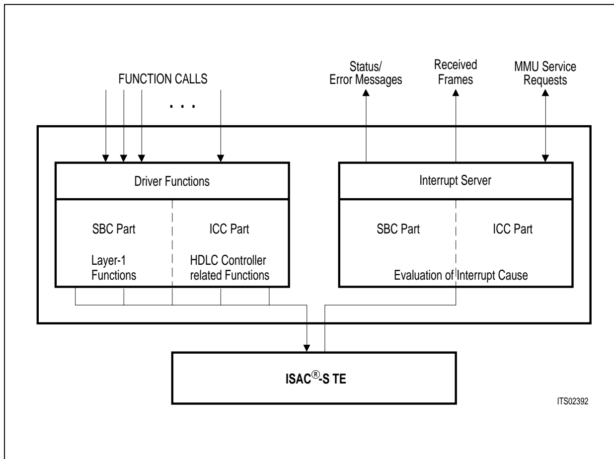
Figure 112 LLC Architecture
