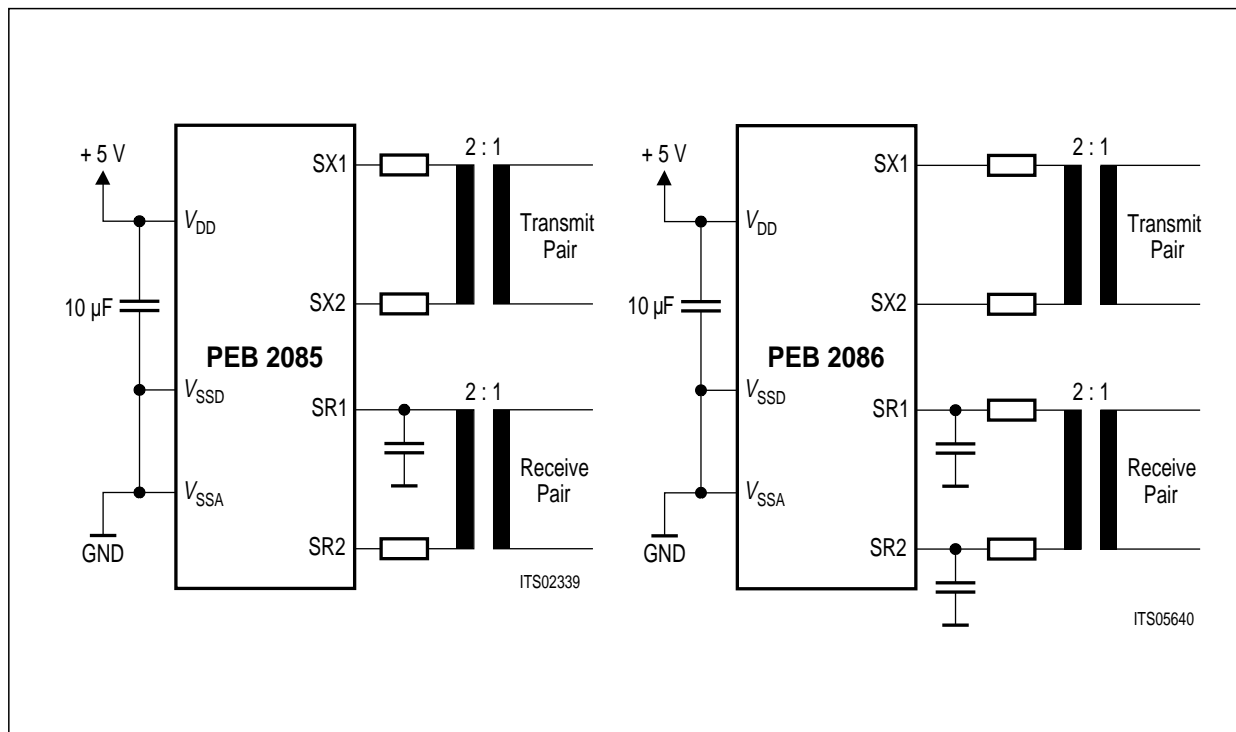
Figure 44 Connection of the Line Transformers and Power Supply to the ISAC®-S
