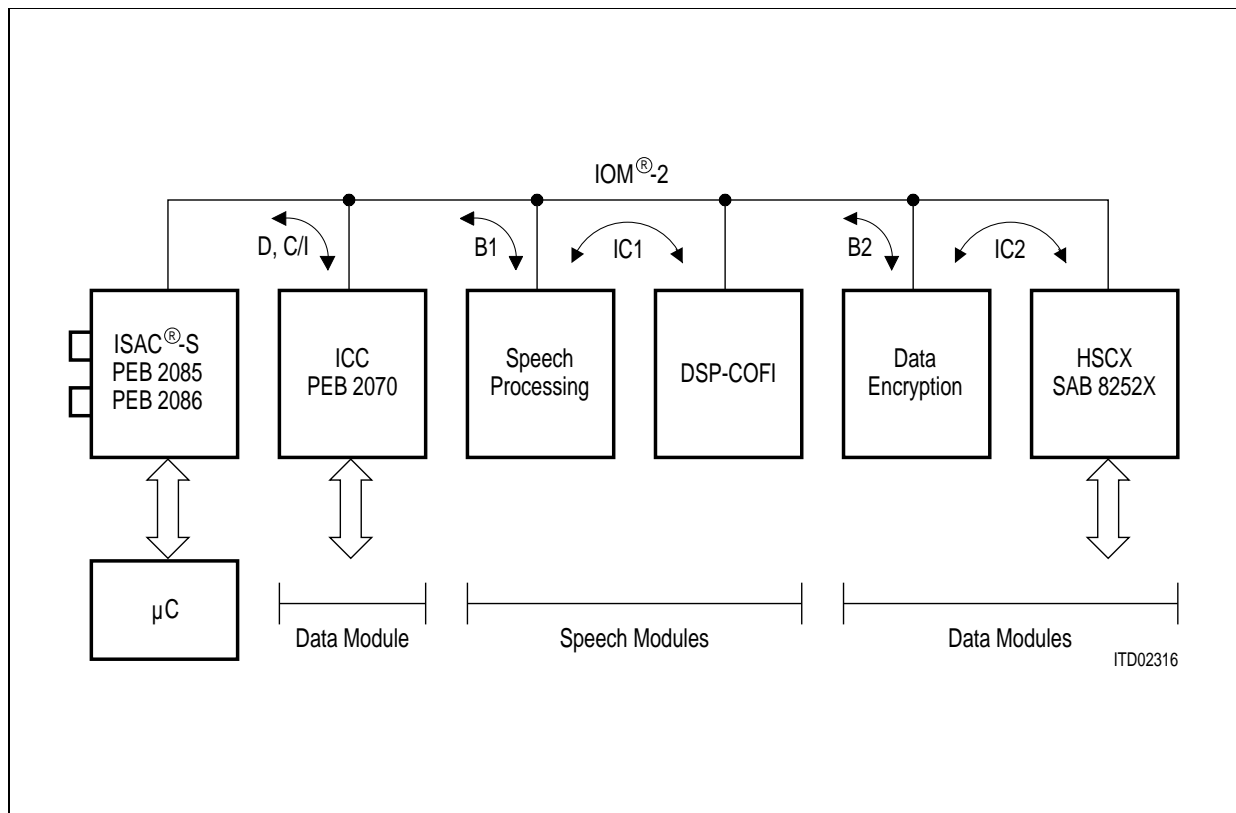
Figure 6 Example of an ISDN ® -S Voice/Data Terminal
