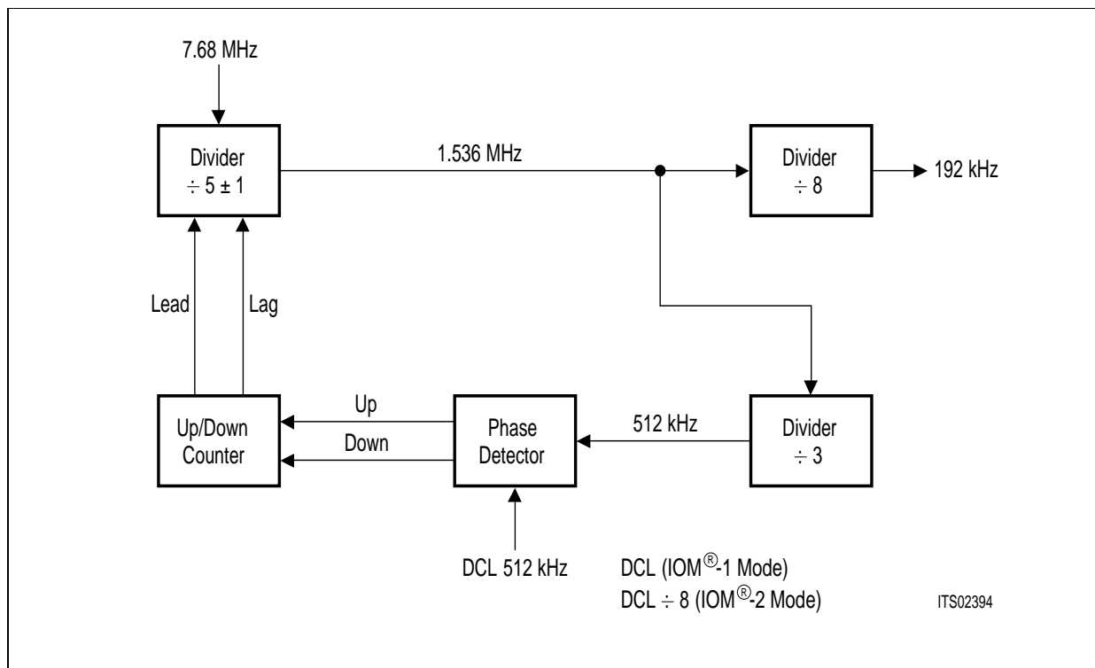
Figure 104 Block Diagram of XPLL
