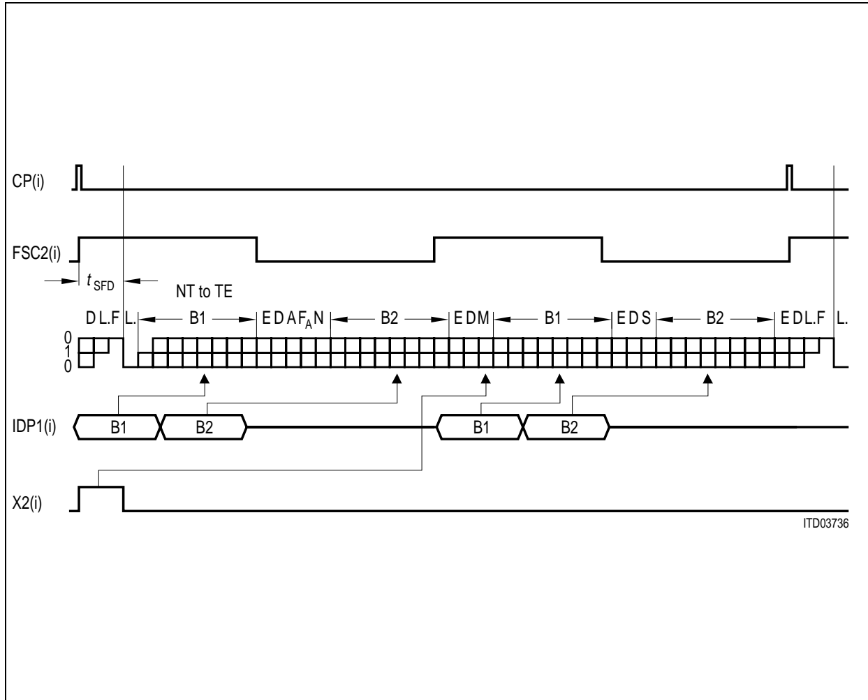
Figure 109 Frame Relationship in Timing Mode 0
