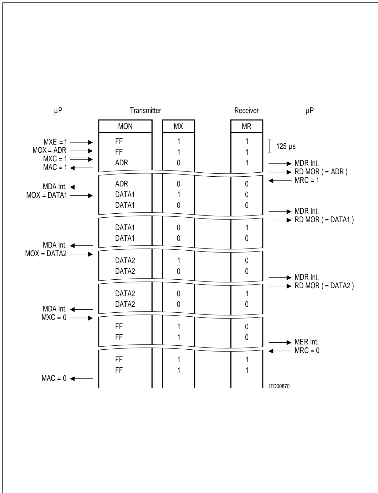
Figure 37 MONITOR Channel Protocol (IOM ® -2)
