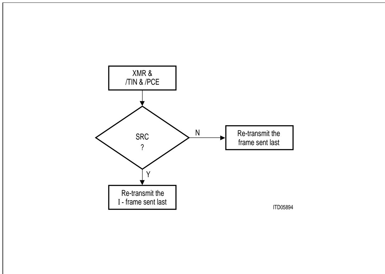
Figure 64 Interrupt Service Routine after XMR
