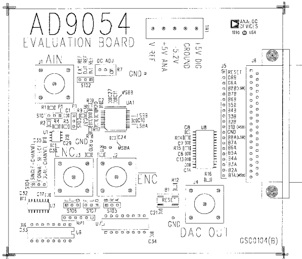
Figure 39. Assembly—Top View
