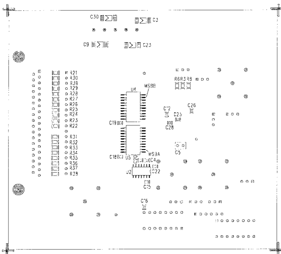
Figure 40. Assembly—Bottom View
