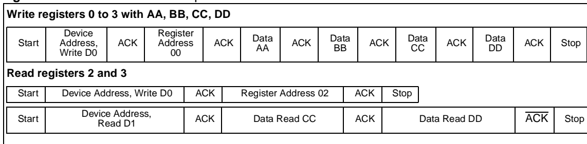
Figure 3: I 2 C Read and Write Operations in Standby Mode
